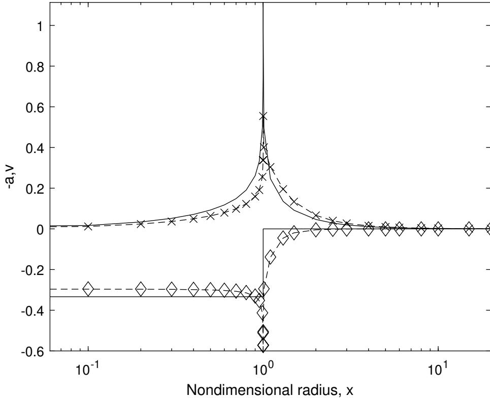
Figure 4. Axial induction, a , and radial velocity, v , for the conditions in Table 1. p = 0.05 : a, \diamond; v, \times . The corresponding results for p = 0.10 are shown as dashed lines. Note that -a is shown to make it distinct from v . The solid lines show a and v for no expansion, i.e. k = 0 , R_\infty = 2 . The x -axis is logarithmic.
