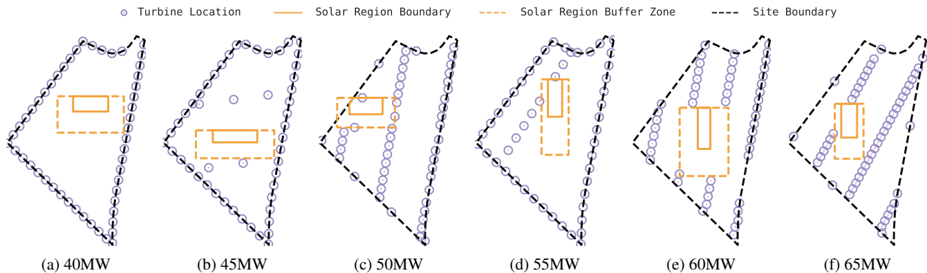
Figure 11. Solutions generated for the high-correlation location and irregular boundary for a range of interconnect capacities, maximizing mean interconnect utilization instead of AEP.
