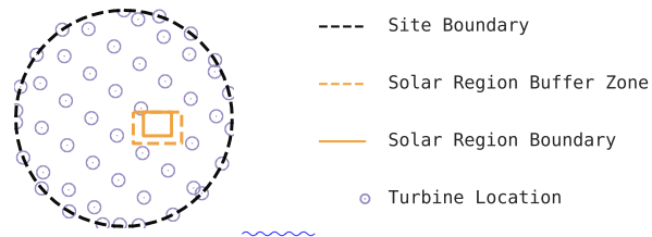
Figure 1. An example layout of a wind-solar hybrid power plant inside a circular site boundary.
