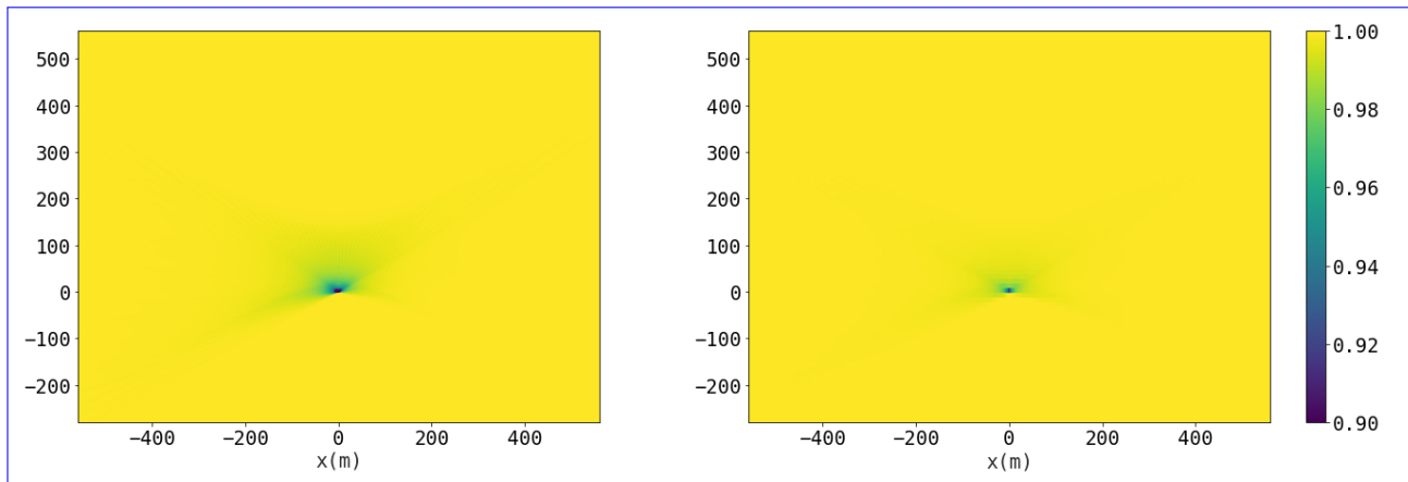
Figure 3. Heat maps of POA loss (left) and PV power loss (right) for a year at (33.209^\circ, -108.283^\circ) , simulated at 15-minute intervals with 12 blade angles per step for a 77 meter diameter turbine at (0, 0).
