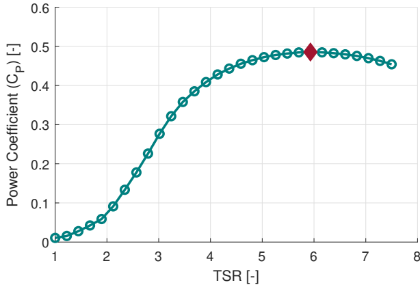
(a) Example of C_P vs TSR curve for Stage 1.
