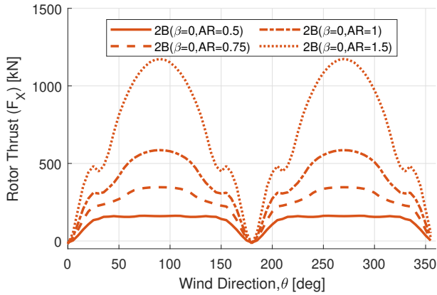
(a) Parsed thrust load ( F_X ) for 2-bladed (2B) rotors.
