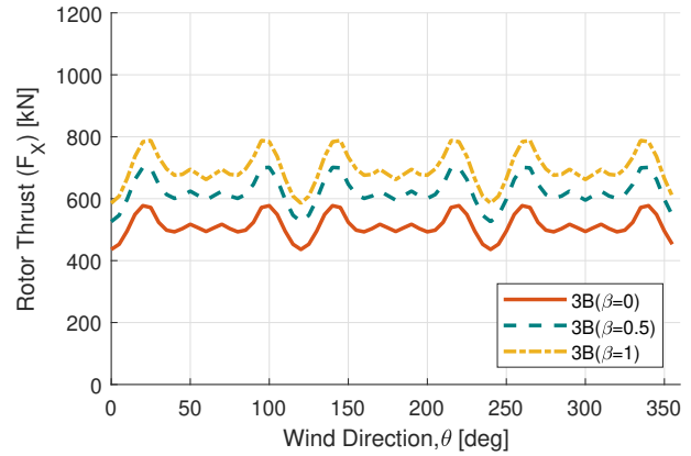
(b) Parsed thrust load ( F_X ) for 3-bladed (2B) rotors
