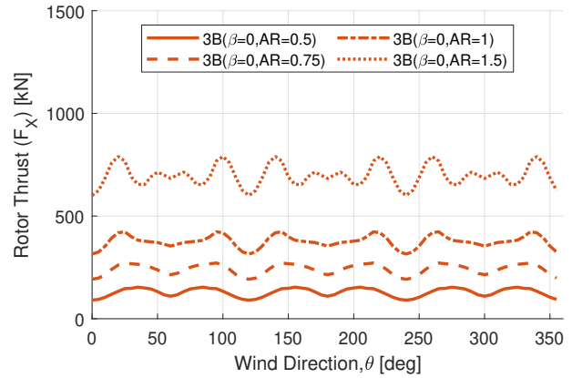
(b) Parsed thrust load ( F_X ) for 3-bladed (3B) rotors.
