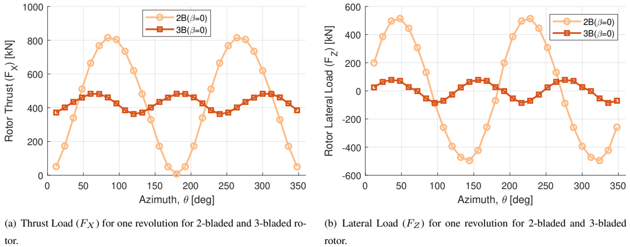
Figure 16. Thrust Load ( F_X ) and Lateral Load ( F_Z ) for one revolution for 2-bladed and 3-bladed turbine.
