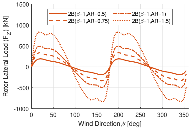
(a) Parsed lateral load ( F_Z ) for 2-bladed (2B) rotors.
