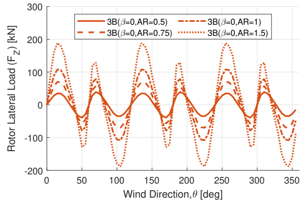
(b) Parsed lateral load ( F_Z ) for 3-bladed (3B) rotors.
