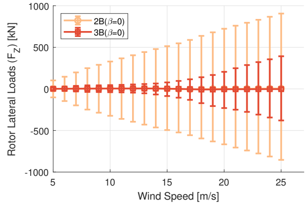
(b) Lateral Load ( F_Z ) vs Wind Speed
