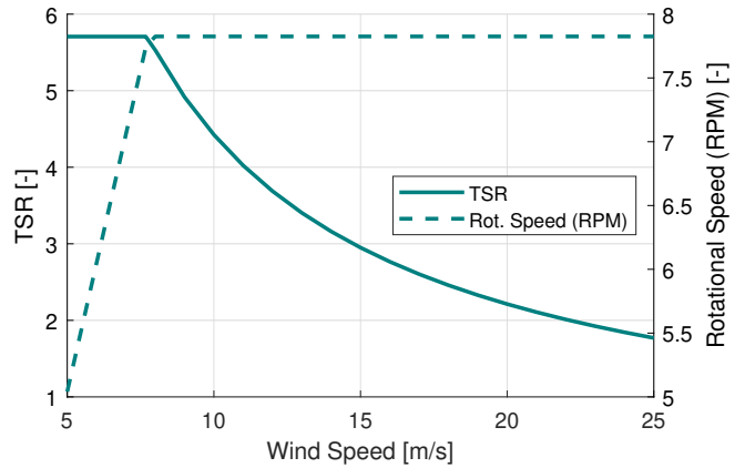
(b) Rotor speed schedule example (Stage 3).
