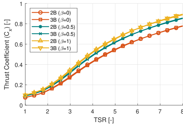
Figure 15. Rotor thrust coefficient ( C_X ) analysis for both 2-bladed (2B) and 3-bladed (3B) rotors.
