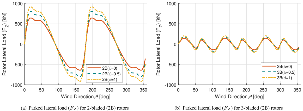
Figure 13. Parked lateral load ( F_Z ) analysis for 2-bladed and 3-bladed rotors.
