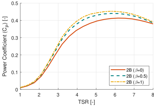
(a) Power coefficient ( C_P ) vs TSR curve for 2-bladed (2B) rotors.
