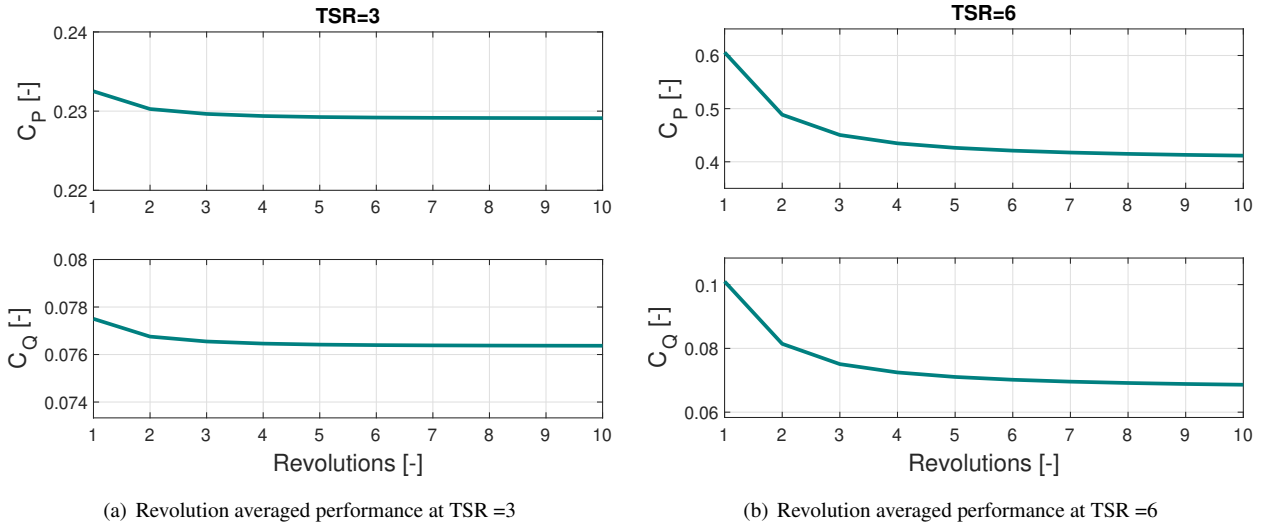
Figure 2. Revolution averaged performance for 10 revolutions at (a) low TSR and (b) high TSR.
