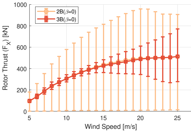
(a) Thrust Load ( F_X ) vs Wind Speed
