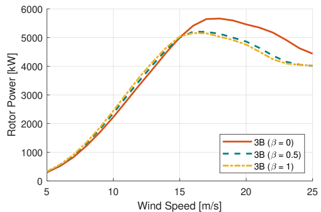
(b) Power vs Wind Speed curve for 3-bladed (3B) rotors.
