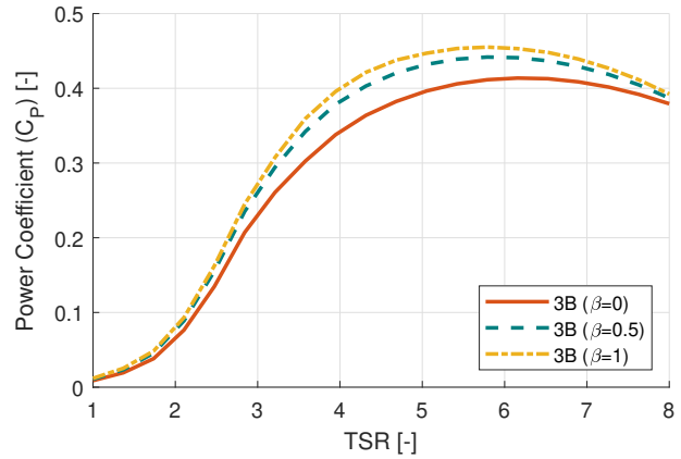
(b) Power coefficient ( C_P ) vs TSR curve for 3-bladed (3B) rotors.
