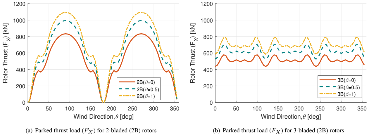
Figure 12. Parked thrust load ( F_X ) analysis for 2-bladed and 3-bladed rotors.
