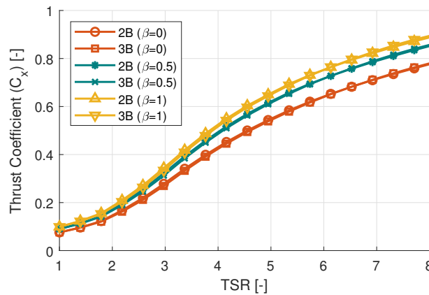
Figure 15. Parked loads comparison with existing literature.
