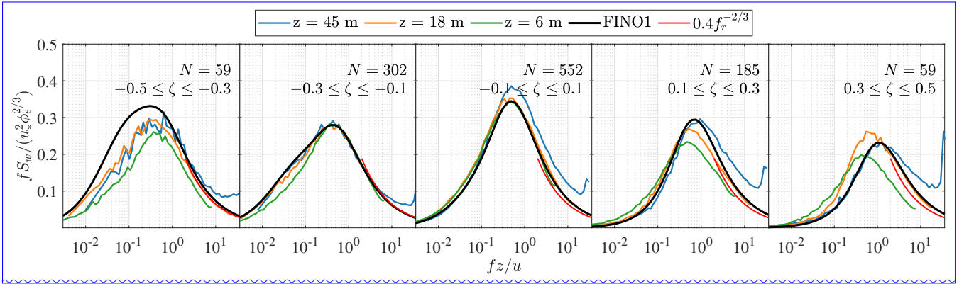
Figure 10. Normalised spectra of the vertical wind component at 45, 18, and 6 m amsl for various stability conditions. The red curve is derived from eq. (6) and N denotes the number of samples considered for ensemble averaging.
