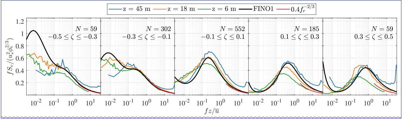
Figure 9. Normalised spectra of the cross-wind component at 45, 18, and 6 m amsl for various stability conditions. The red curve is derived from eq. (6) and N denotes the number of samples considered for ensemble averaging.
