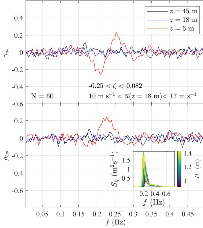
Figure 7. Co-coherence \gamma_{\eta w} and quad-coherence \rho_{\eta w} between the velocity of the wave surface \dot{\eta} and the vertical wind velocity w from the three sonic anemometers on SMW. The inset shows the individual wave elevation spectra S_{\eta} associated with H_s > 0.9 m (60 samples) used to estimate \gamma_{\eta w} and \rho_{\eta w} .
