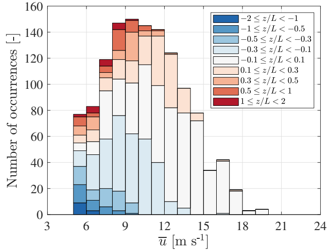
Figure 6. Stability distribution as a function of mean wind speed for the considered feteh -fatches (220°-330°) at height z = 18 m.
