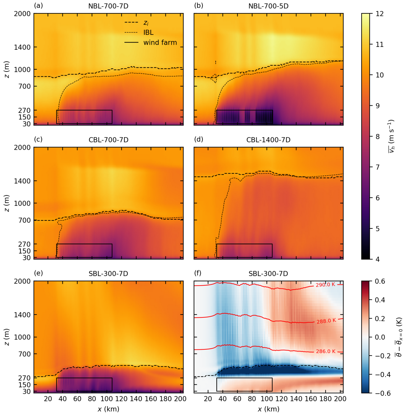
Figure 7. Vertical cross sections at y = 120 km of wind speed v_h for all cases (a-e) and potential temperature deviation relative to the inflow temperature for case SBL-300-7D (f). The Also shown are the inversion layer height z_i is marked by a line that marks the (maximum vertical temperature gradient), the internal boundary layer IBL (97 % of inflow wind speed) and the extend of the wind farms in Zone 3.
