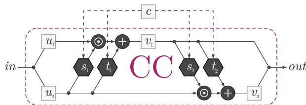
Figure 3. The conditional coupling blocks CC with its embedded sub-network s_1, t_1, s_2, t_2 . This CC architecture can easily be inverted. Ardizzone et al. (2019b)
