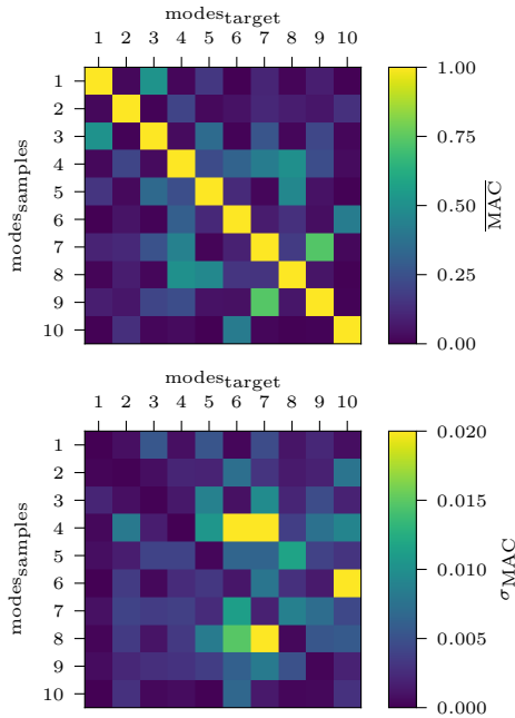
Figure 16. Mean values (top) and standard deviations (bottom) of the MAC matrix for the free-free modal configuration based on 1,000 spline samples inferred for one target response.
