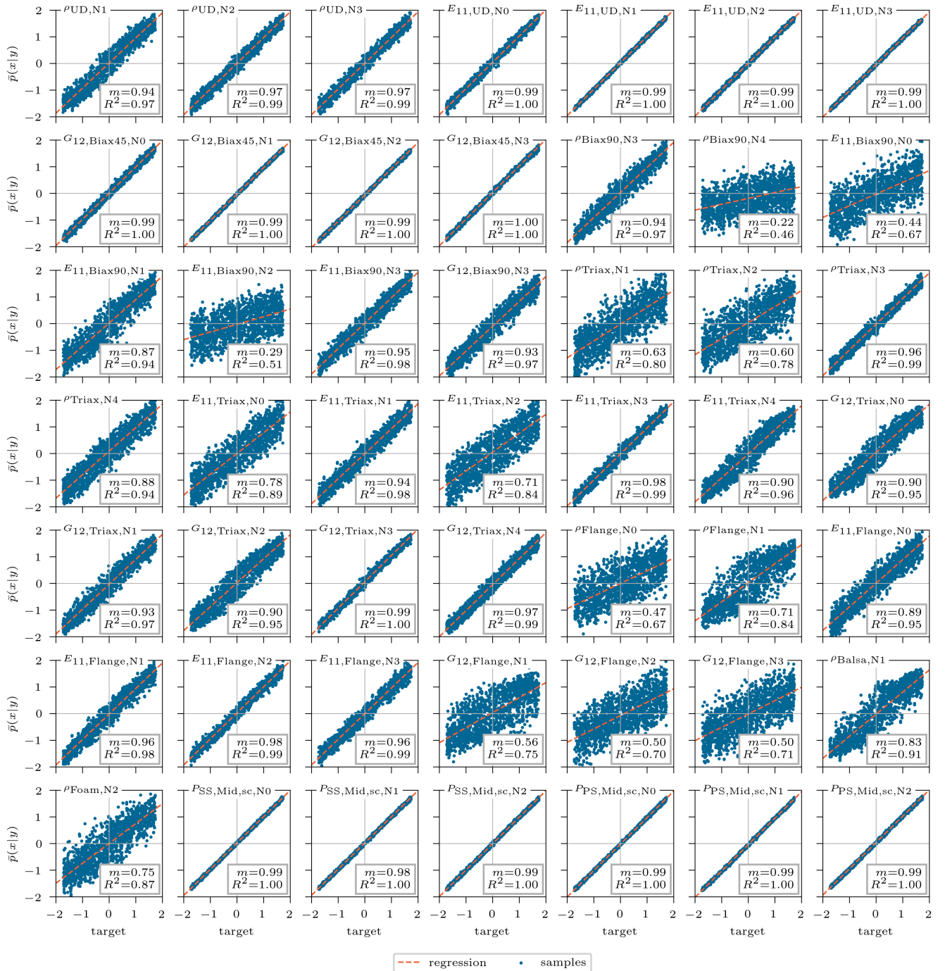
Figure 9. Standardized mean of posterior prediction \bar{x} of the updated inputs over the corresponding target standardized value for the 5,000 test samples. The coefficient of determination and a corresponding linear regression line are shown. The corresponding parameter description to the features can be found in Table 2.
