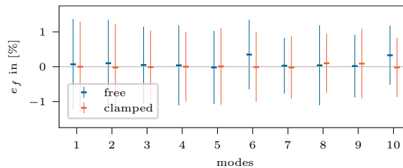
Figure 18. Mean and standard deviation of the natural frequency error e_f computed for 1,000 target responses.
