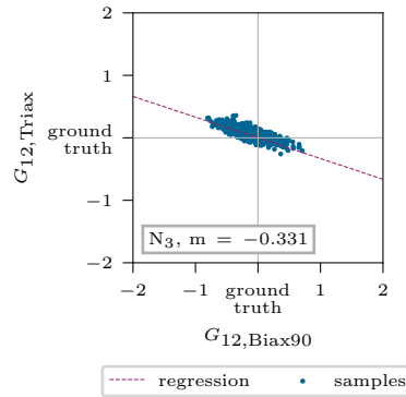
Figure 12. Interaction of shear stiffness G_{12,Biax90} and G_{12,Triax} describing the intrinsic model ambiguities. The depicted values correspond to the standardized mean posterior prediction for the 5,000 test samples.
