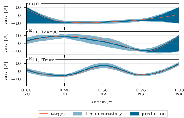
Figure 15. Exemplary inferred spline prediction range for \rho_{UD} , E_{11, Biax90} and E_{11, Triax} . The graphs depict the target spline in orange, the mean prediction in dark blue, and the 1\text{-}\sigma -uncertainty in light blue, for the updated spline nodes.
