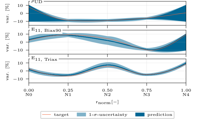
Figure 15. Exemplary inferred spline prediction range for \rho_{UD} , E_{11,Biax90} and E_{11,Triax} . The graphs depict the target spline in orange, the mean prediction in dark blue, and the 1-\sigma -uncertainty in light blue, for the updated spline nodes.
