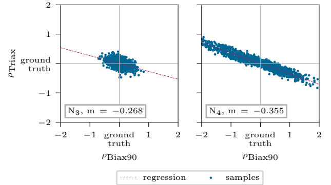
Figure 10. Interaction of density \rho_{\text{Biax}90} and \rho_{\text{Triax}} describing the intrinsic model ambiguities. The depicted values correspond to the standardized mean posterior prediction for the 5,000 test samples.
