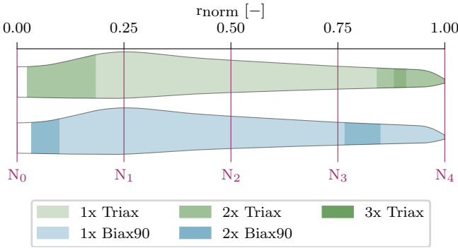
Figure 14. Layout of the sandwich laminate face sheets of the blade shell, consisting of Triax and Biax90°. The inner and outer face sheets are symmetric.
