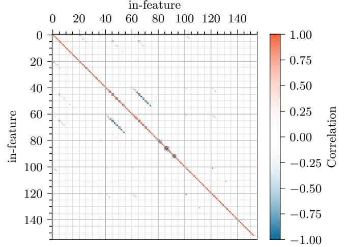
Figure 19. Cross-correlation of all input feature based on mean posterior prediction of the 5,000 test samples.
