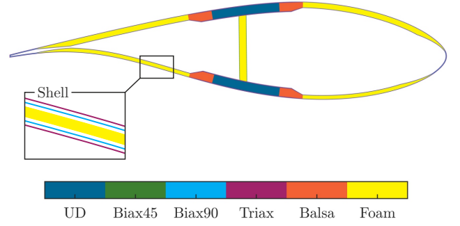
Figure 13. Schematic blade cross-sectional view at a radial position of r = 12 m with a detailed explosion drawing of the shell.
