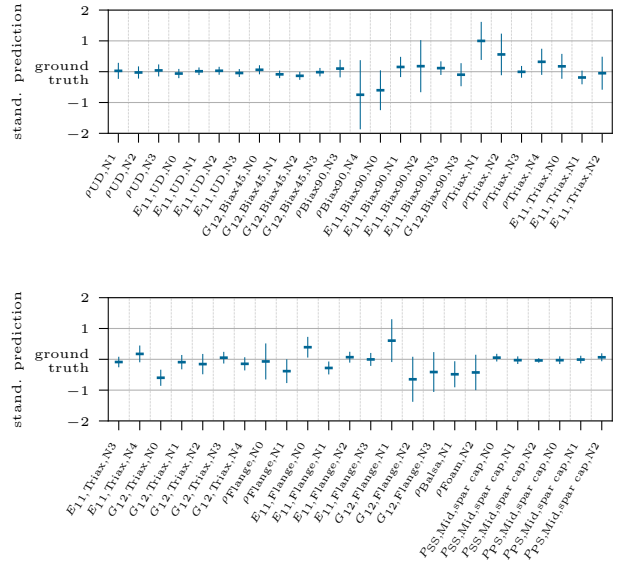
Figure 8. The first two graphs show the standardized posterior prediction for all updated input features related to the target value with 1- \sigma standard deviation as error, thus the mean value marks the distance to the target value, i.e., ground truth.
