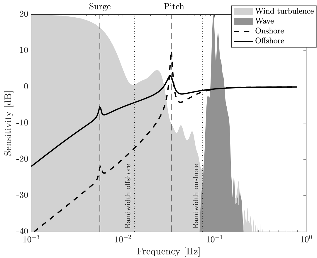
Figure 1: The sensitivity function of the blade-pitch feedback controller with original (Onshore) and detuned (Offshore) gains. In the background, it is shown the typical PSD of wind and waves, which magnitude has been rescaled to ease the comparison with sensitivity functions.
