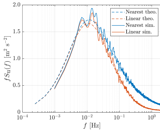
Figure 8. Comparison of the impact of nearest-neighbor interpolation and linear interpolation on the auto-spectrum of the u component. A 2-by-2 square grid on the yz plane with a width of 5 m is considered and the point to be interpolated is the center point of the square grid. The auto-spectra are averaged with 16 samples.
