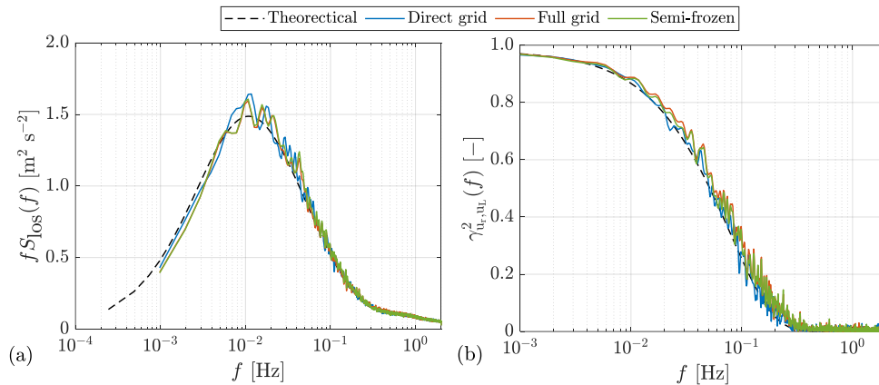
Figure 10. Comparison of the simulated spectral properties with different grids. Direct grid: all the points required for lidar simulations are directly defined in the 4D wind field generation. Full grid: the vertical planes with regular grid points at the x positions of the focus points and the discrete volumes of the lidar range gates. Semi-frozen: the vertical planes with regular grid points at the x positions of the focus points of the lidar range gates. Beam azimuth angle: 15.0^\circ . Beam elevation angle: 12.5^\circ . Range gate: 87 m. The simulated auto-spectra are averaged with 16 samples.
