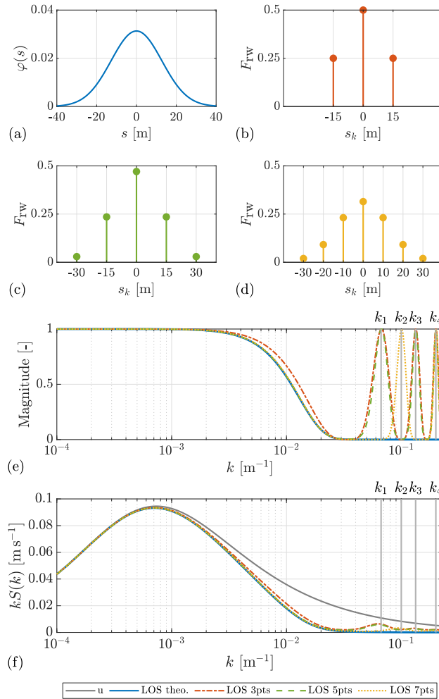
Figure 6. (a) Theoretical Gaussian-shape range weighting function with a full width at half maximum of 30 m for a pulsed lidar. (b-d) 3-point, 5-point, and 7-point normalized discrete approximations of the range weighting function, with steps \Delta s_k of 15 m, 15 m, and 10 m, respectively. (e) Magnitudes of the FFTs of the different discretizations of the range weighting function. Critical wavenumbers: k_1 = 1/15 \text{ m}^{-1} , k_2 = 1/10 \text{ m}^{-1} , k_3 = 2/15 \text{ m}^{-1} , k_4 = 1/5 \text{ m}^{-1} . (f) Theoretical auto-spectra of the u component and the LOS measurements of the different discretizations of the range weighting function. The LOS measurements are assumed aligned to the wind direction.
