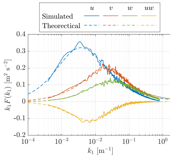
Figure 5. Comparison of the simulated and theoretical spectra of the Mann (1994) model at x = 100 m in a 4D wind field. The simulated spectra are averaged with 16 samples.
