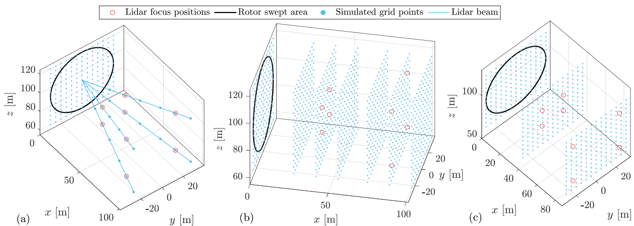
Figure 9. Illustration of three types of grids for lidar simulations. (a) Direct grid. (b) Full grid. (c) Semi-frozen grid.
