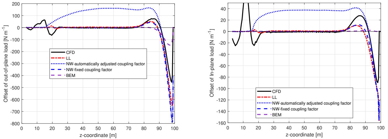
Figure C6. Comparison of the difference between the out-of-plane load (left) and the in-plane load (right) of the forward swept Blade-8 with respect to the baseline blade calculated from the Navier-Stokes solver (CFD), the lifting-line method (LL), the proposed coupled method (NW) and the blade element momentum method (BEM).
