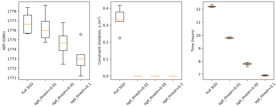
Figure 8. Results using different configurations of the “early stopping” option in TOPFARM, as well as the “SGD optimization without early stopping, considering the circular wind farm with 225 turbines, with T = 2,000 , using five random initial layouts.
