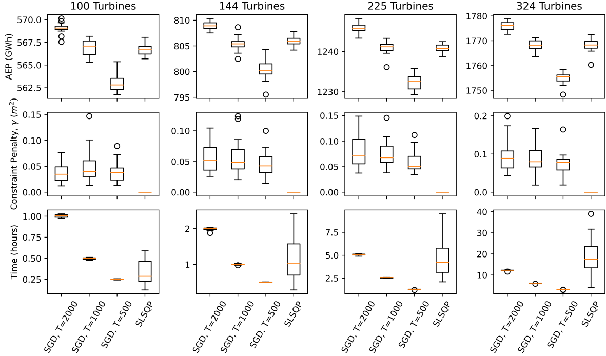
Figure 4. Optimization results associated with SGD and SLSQP for square wind farms with 100, 144, 225, and 324 turbines, using 20 random initial starting conditions. The AEP (top panel), constraint penalty (middle panel), and computational time (bottom panel) are plotted as boxplots. The SGD results are plotted for T = 500, 1,000, and 2,000 iterations.
