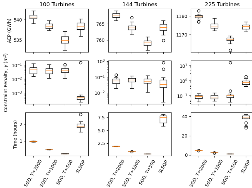
Figure 6. Optimization results associated with SGD and SLSQP for wind farms with 100, 144, and 225 turbines, using 20 random initial starting conditions. The AEP (top panel), constraint penalty (middle panel), and computational time (bottom panel) are plotted as box and whisker plots. The SGD results are plotted for T = 500, 1,000, and 2,000 iterations.
