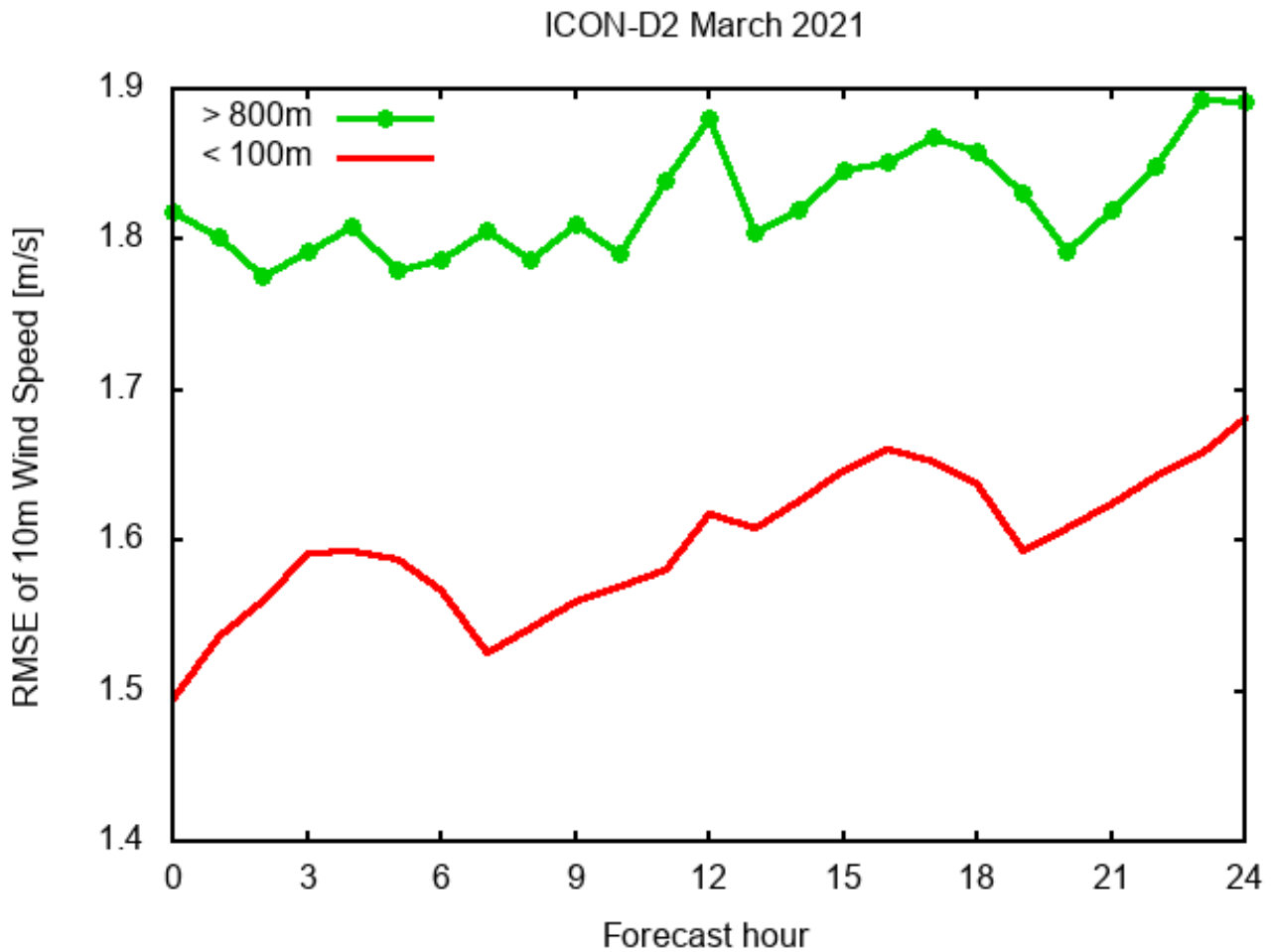
Figure 3. RMSE of 10 m wind speed from the numerical weather prediction model ICON-D2 in March 2021 compared to observations at sites below 100m (red) and above 800 m a.s.l. (green). The ICON-D2 domain covers central Europe including most of France to Poland, and from northern Italy to Denmark and thus locations above 800 m are typically in hilly or mountainous terrain. For details of the ICON-D2 model, see ?.
