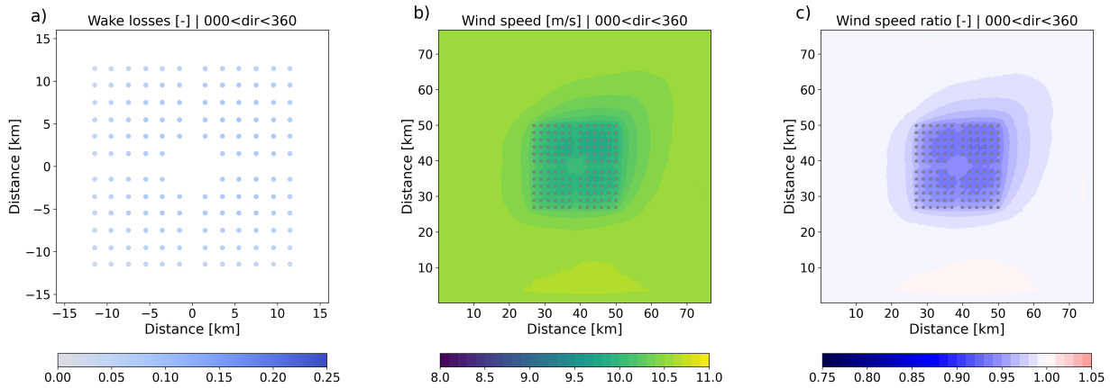
Figure 14. As Fig. 13, but for the 5 \text{ MW km}^{-2} scenario (including all data).
