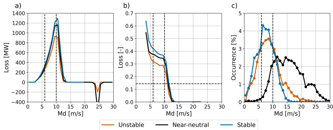
Figure 7. Combined effect of wind speed and stability on wind farm aerodynamic losses. a) Power losses in MW. b) Fractional-Relative aerodynamic losses. c) Frequency of occurrence of the three stability classes. Dashed lines at 6 and 10 \text{m s}^{-1} indicate the wind speed interval for which the aerodynamic losses are relatively constant.
