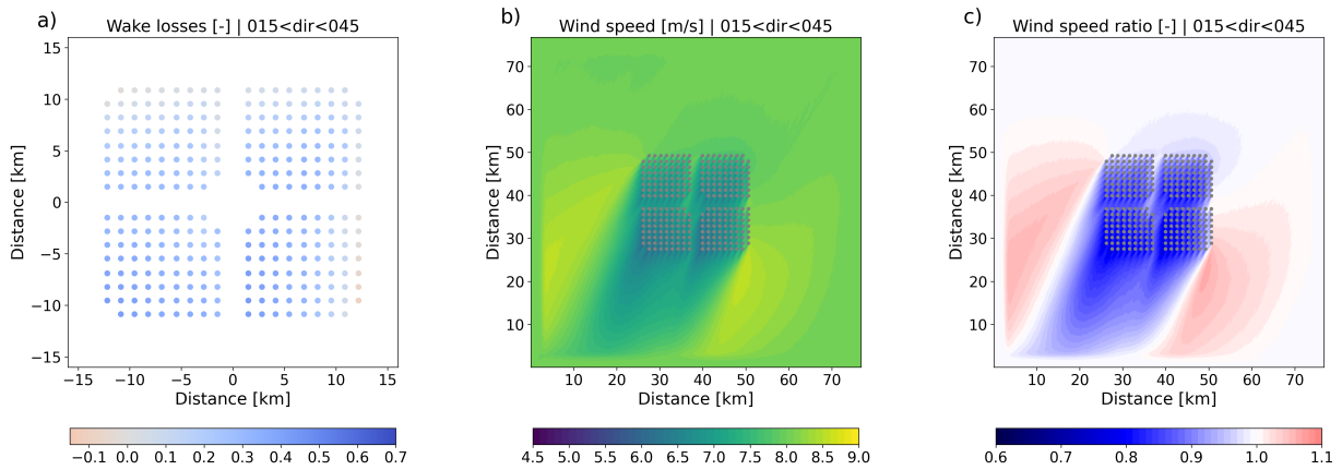
Figure 18. As Fig. 13, but only including unstable-convective conditions, wind speeds between 6 and 10 \text{ms}^{-1} , and wind directions between 15 and 45 degrees.
