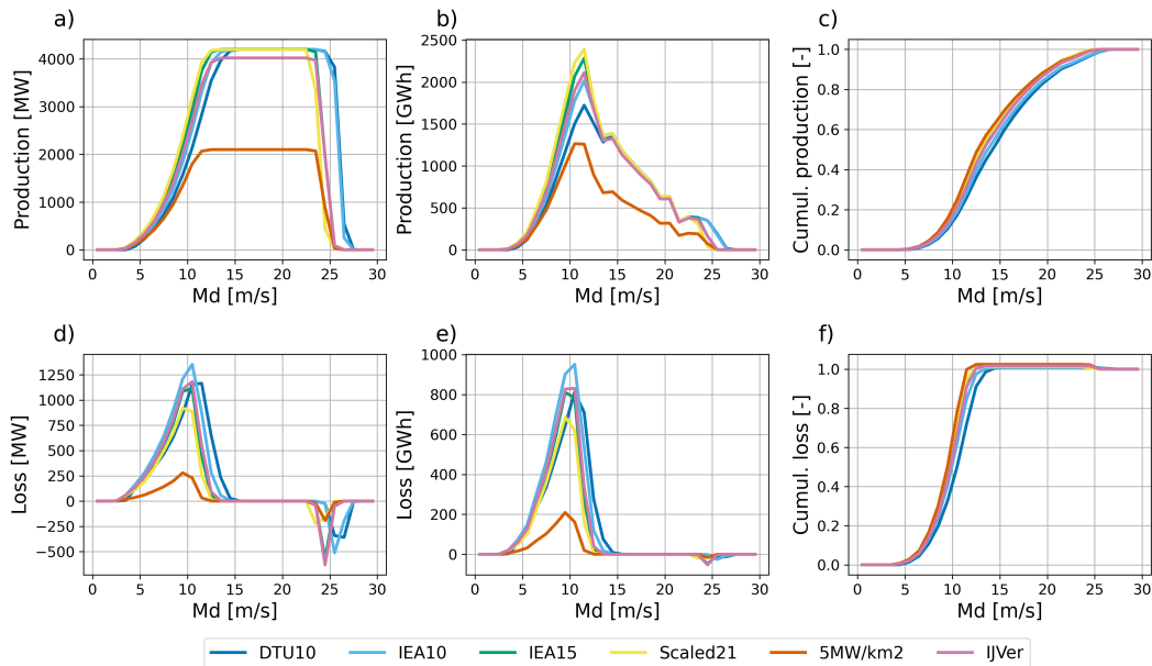
Figure 6. Top: year-averaged wind farm power production (a), total energy production for 1 m s -1 bins (b), and normalized cumulative production (c) as function of the free-stream disk-averaged wind speed. Bottom: year-averaged wind farm power losses (d), total aerodynamic losses for 1 m s -1 bins (e), and normalized cumulative losses (f) as function of the free-stream disk-averaged wind speed.
