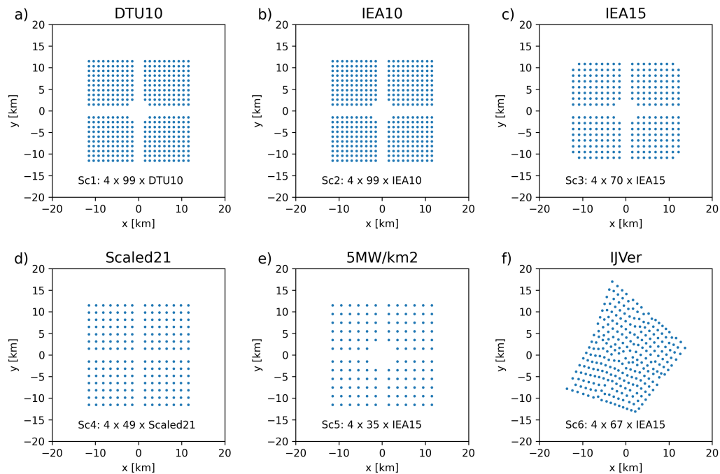
Figure 3. Layouts of the six 4-wind farm scenarios. Panel titles refer to the scenario labels in Table 1. For each scenario the number and type of the applied turbine is indicated.
