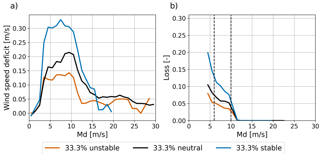
Figure 10. Dependence of the reduction of the first-row 140 m wind speed deficits and first-row production losses as a function of wind speed and stability. a) Reduction in wind speed of first-row turbines compared to the free stream wind speed. b) First-row and the relative aerodynamic losses of first-row turbines. Frequency as a function of occurrence wind speed and stability.
