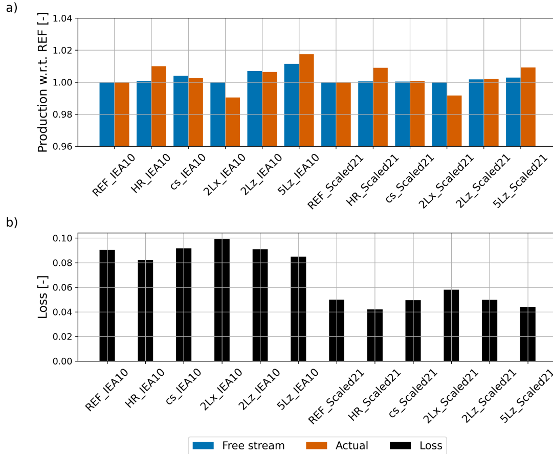
Figure 20. Fractional difference in both thrustless Free stream and actual production between of the sensitivity experiments and with respect to REF (a) Aerodynamic and the corresponding aerodynamic losses (b).
