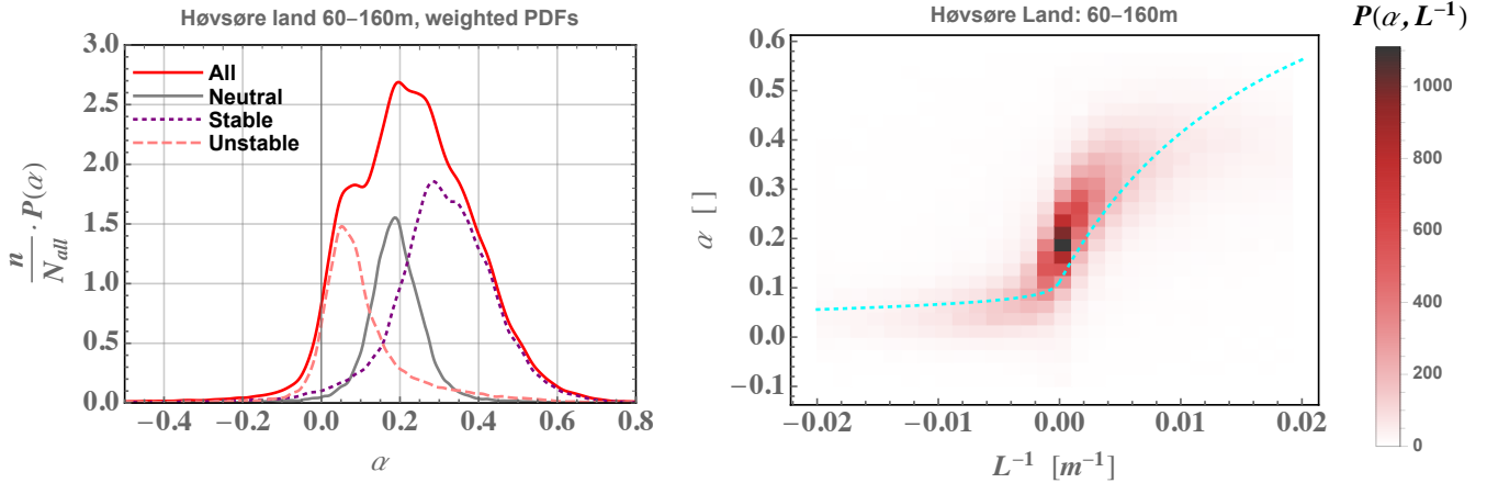
Figure 7. Left: PDF of shear exponent \alpha , weighted by frequency of occurrence for different atmospheric stability conditions; neutral defined by |L^{-1}| < 0.001\text{m}^{-1} , stable has L^{-1} > 0.001\text{m}^{-1} , and unstable has L^{-1} < -0.001\text{m}^{-1} . Right: joint PDF of shear exponent calculated from 60–160 m height and inverse Obukhov length (surface-layer stability) at z = 10 m from sonic anemometers over the homogeneous land sectors at Høvsøre, along with M-O similarity implied by (2) shown by dashed cyan line; JPFD value of 1000 corresponds to approximately 3.5% occurrence. Measurements span one decade, starting 2005.
