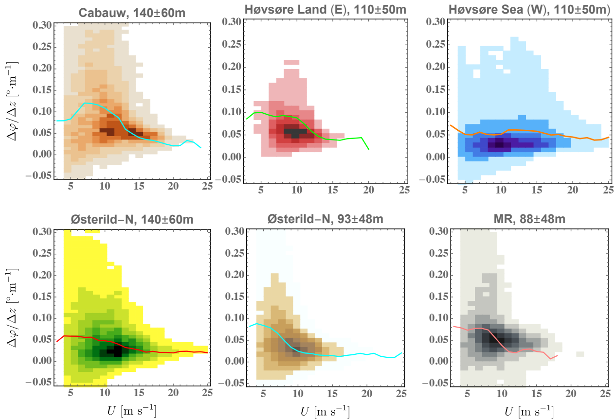
Figure 11. Joint distribution of veer and wind speed at sites considered. Solid line shows \langle \Delta\phi/\Delta z \rangle|U , calculated using 1 \text{ m s}^{-1} bins; lightest shades are 2% as likely as darkest color in each plot.
