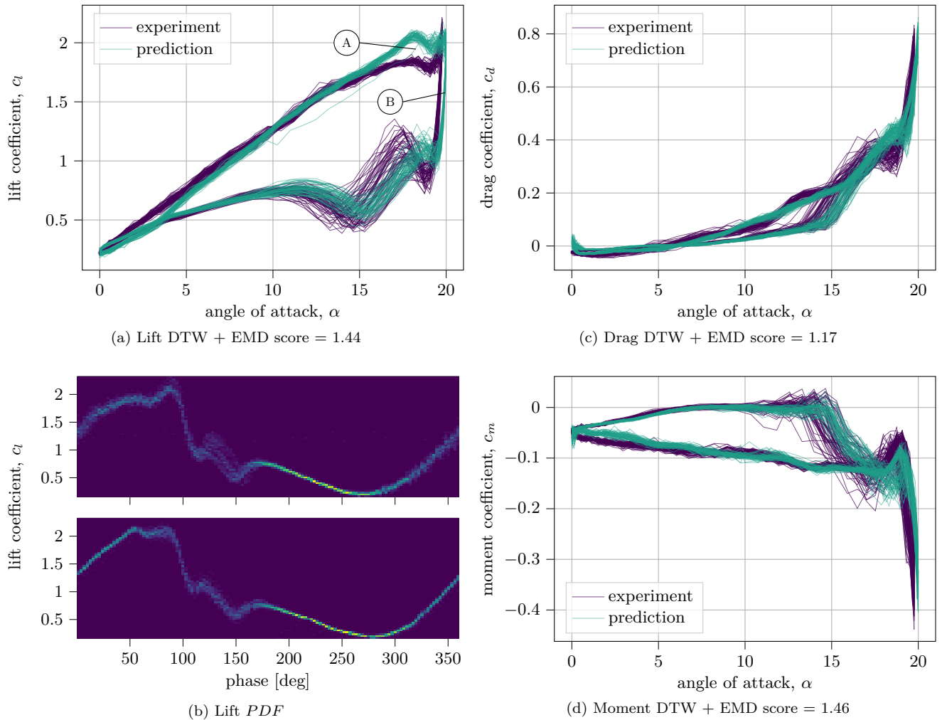
Figure 9. Unsteady aerodynamic coefficients with gusts under dynamic stall conditions in comparison with the experimental results for the parameters f = 1.20 Hz, \alpha_m = 10^\circ , \alpha_a = 10^\circ , Re = 300000 \pm 50\% , \tau = 90^\circ . The DTW + EMD score score indicates how close the two distributions are for each individual coefficient (smaller is better). 60 cycles are predicted. ?? shows the global probability density function of the experiments (top) and predictions (bottom) for the unwrapped lift case in phase space.
