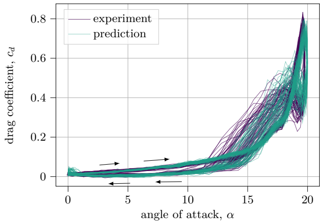
(c) Drag DTW + EMD score = 1.12
