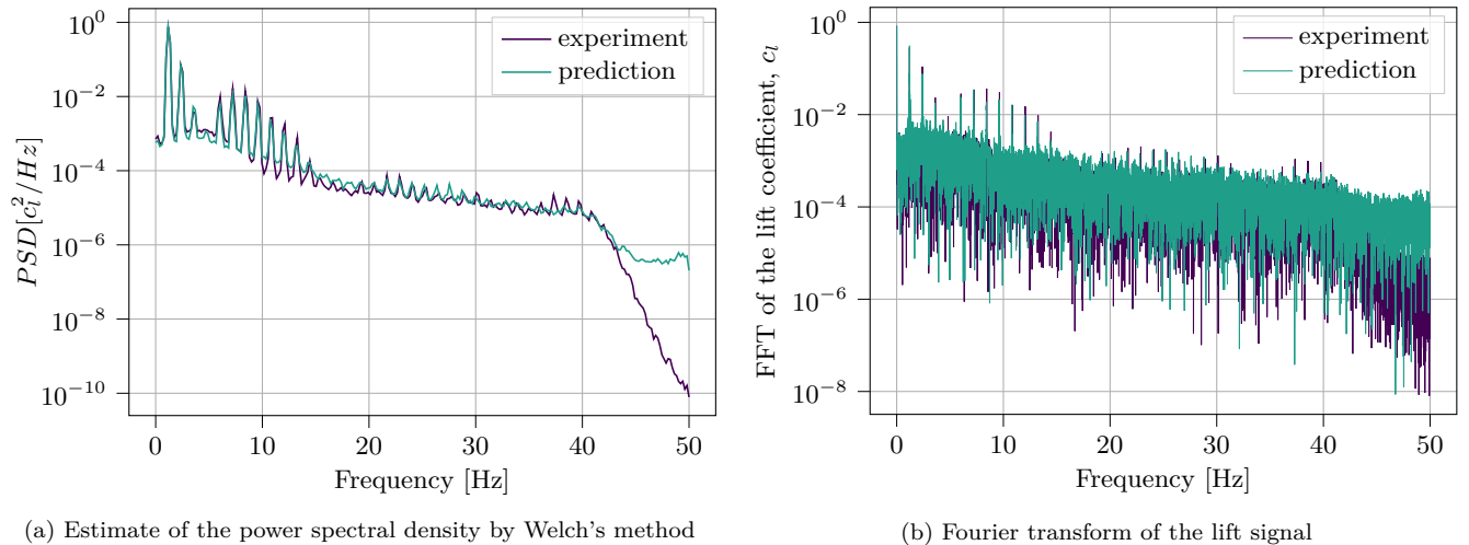
Figure 11. Frequency response analysis for the S809 airfoil with the parameters f = 1.2\text{Hz} , \alpha_m = 10^\circ , \alpha_a = 10^\circ and Re = 300000
