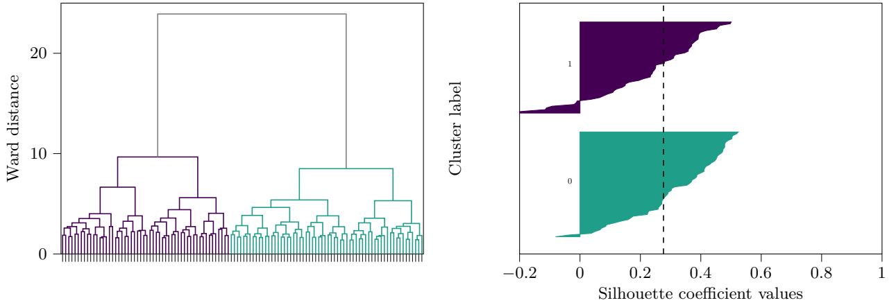
(a) Dendrogram whose leaves are colored according to the cluster membership, the length of the branches indicates the distance/dissimilarity to the nearest node
