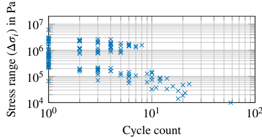
Figure 11. Results of the rainflow cycle count for a ten-minute interval (18 March 2016; 00:10:00). Strain gauge at 225°, which corresponds to side-to-side direction for this interval.
