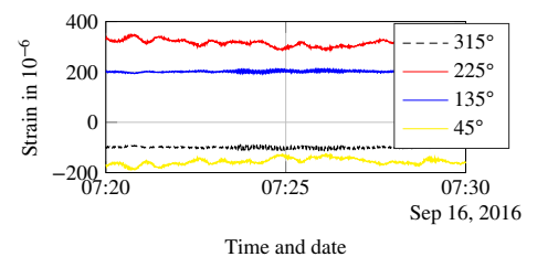
Figure 6. Example strain data. A wind direction of approximately 235° leads to wind-induced oscillations for the sensors at 225° (tension) and 45° (compression) and oscillations in its eigen-frequencies in side-to-side direction (sensors at 135° and 315°).
