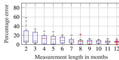
Figure 23. Convergence of the percentage error of predicted damage values using the binning approach for increasing measurement lengths. Box plot shows data from 13 “different” measurement periods.
