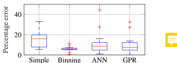
Figure 19. Percentage errors of predicted damage values using all extrapolation methods compared to real damage values. Predictions from one year to a second year for 13 “different” years.
