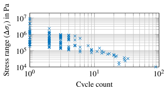
Figure 10. Results of the rainflow cycle count for a ten-minute interval (18 March 2016; 00:10:00). Strain gauge at 315°, which corresponds to fore-aft direction for this interval.
