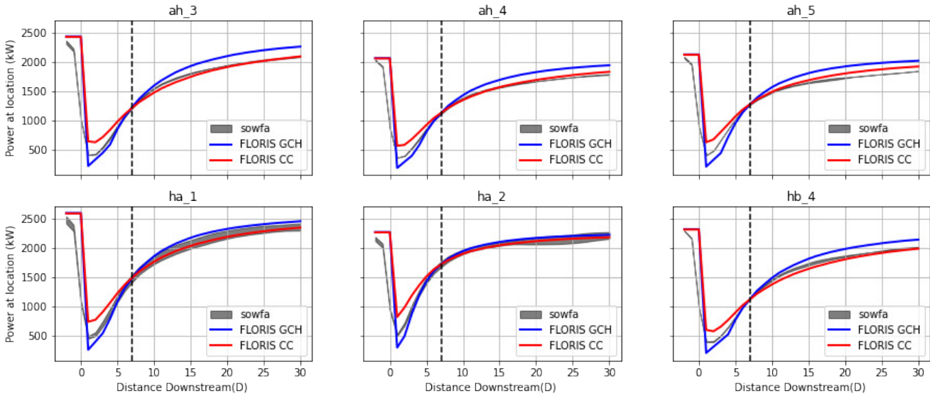
Figure 1. Power production of a downstream wind turbine located at various distances behind a yaw-aligned upstream wind turbine for each precursor described in Table 1. The TI values for both the GCH and CC models were selected to match the wake depth in SOWFA at 7D distance (indicated via a dashed line). Note that empirical results have shown that the GCH model typically overpredicts recovery for distances >10D (Doekemeijer et al., 2022).
