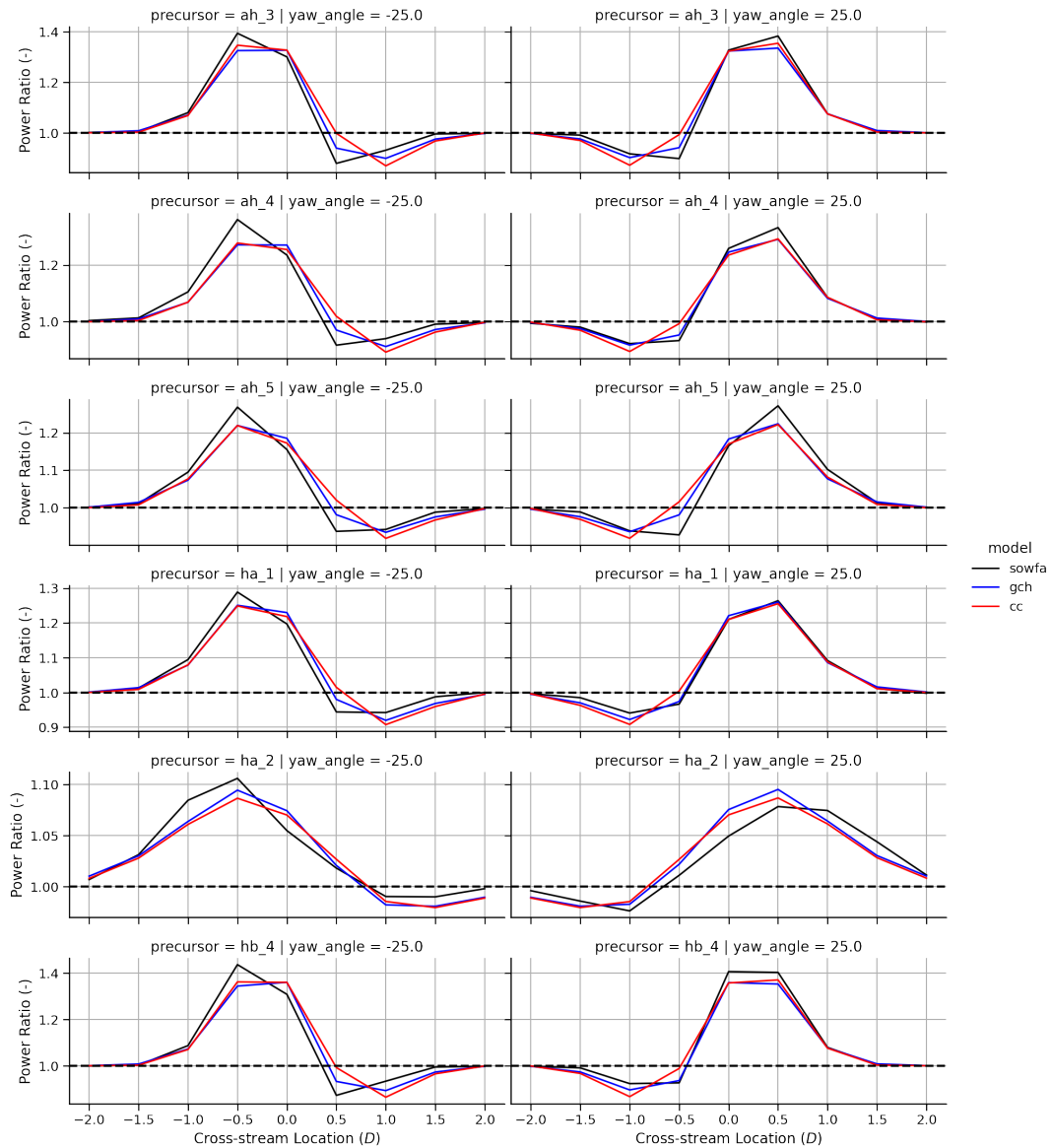
Figure 3. The power production of a hypothetical turbine 7 rotor diameters distance from an upstream wind turbine. The upstream wind turbine is misaligned by 25^\circ in either direction. The left column of subplots compares a -25^\circ (in the clockwise direction) change in yaw to the aligned case, and the right column displays a +25^\circ yaw misalignment (in the counterclockwise direction). The difference between the CC and GCH models for single-turbine wake steering is small, which is reassuring because the GCH model has previously shown good agreement with experimental data (Fleming et al., 2021).
