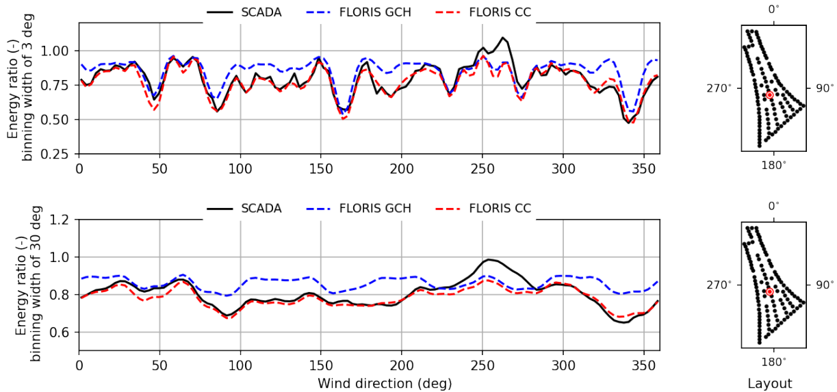
Figure 14. Energy ratio versus wind direction for Turbine 86, located in the center of the Anholt wind farm. The reference turbines to which the energy ratio is normalized are the five closest wind turbines that are operating in freestream flow. The reference wind direction is determined by the nacelle headings from turbines directly neighboring Turbine 86.
