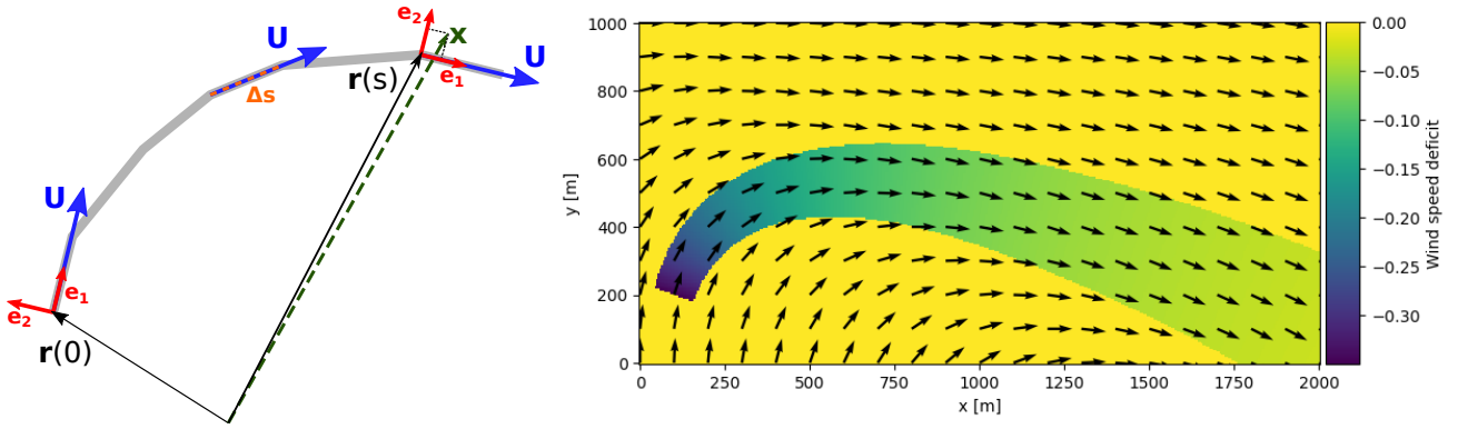
Figure 3. Left: The thick gray line represents the piecewise linear streamline, as obtained from the steady-state flow field U based on the selected time step \Delta t . The wake-causing rotor is located at position r(0) . Each segment has its own local coordinate system, indicated by the red vectors e_1, e_2 . Here x denotes the point of wake model evaluation, and r(s) is the nearest support point of the discretized streamline. Right: An example outcome for the Jensen wake model in a wind field with rotation.
