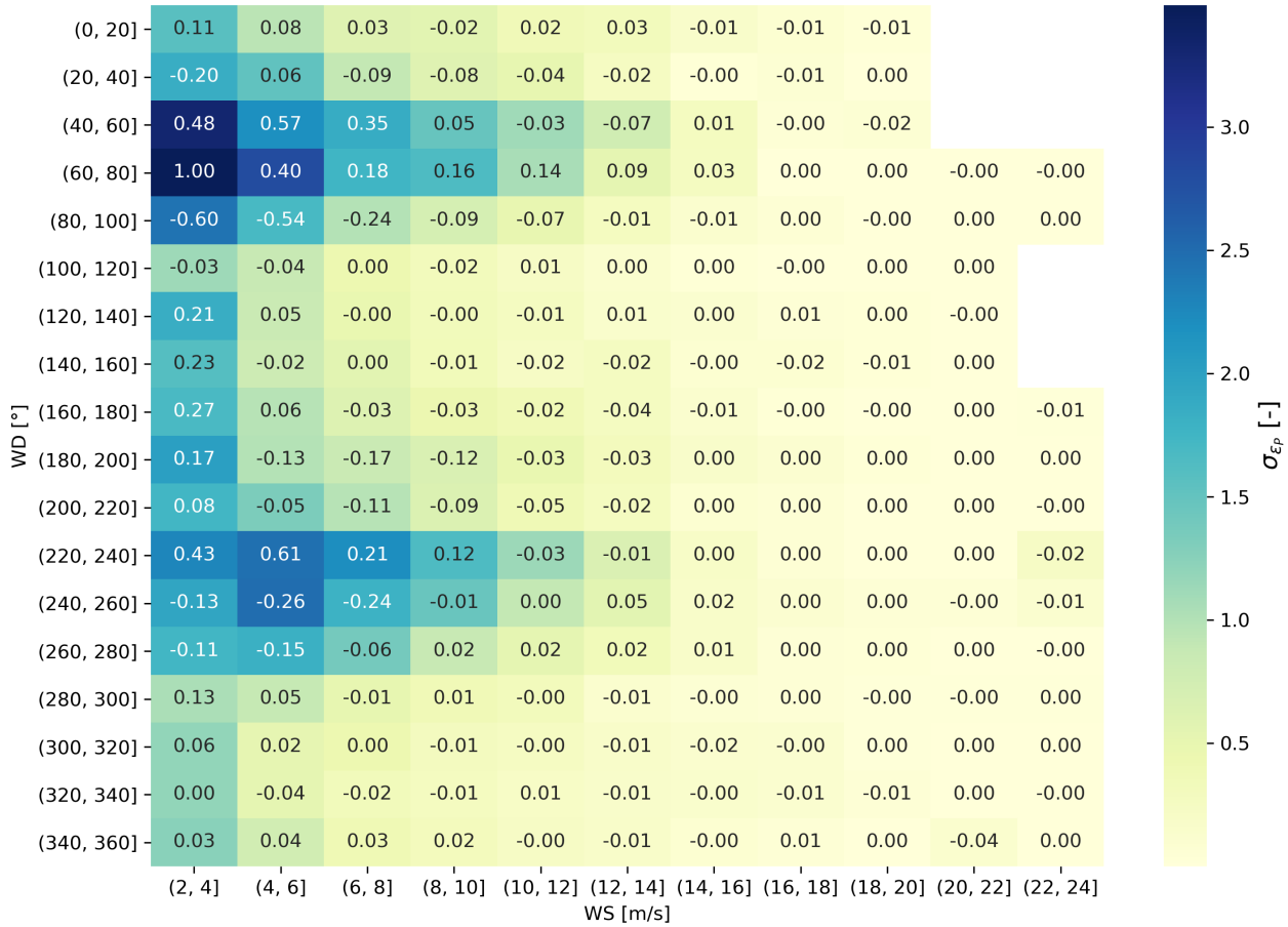
Figure 10. Heatmap of the standard deviation (colors) and mean (annotated number) of the relative difference between the streamline wake model and the baseline model in the calculation of the energy yield of the N6 and N8 cluster. Here, the wind linear superposition was applied. Annotated values are the mean of the same value. The mean and the standard deviation are computed as \mu_{\epsilon_p} = \frac{1}{n} \sum_{i=0}^n (P_{i,N6N8}^{SWM} / P_{i,N6N8}^{BLM} - 1) and \sigma_{\epsilon_p} = \frac{1}{n-1} \sqrt{\sum_{i=0}^n [(P_{i,N6N8}^{SWM} / P_{i,N6N8}^{BLM} - 1) - \mu]^2} , respectively, with n the last time step of the NEWA time series considered. The wind speed and direction considered for the bin is taken from easternmost turbine row of the cluster N6.
