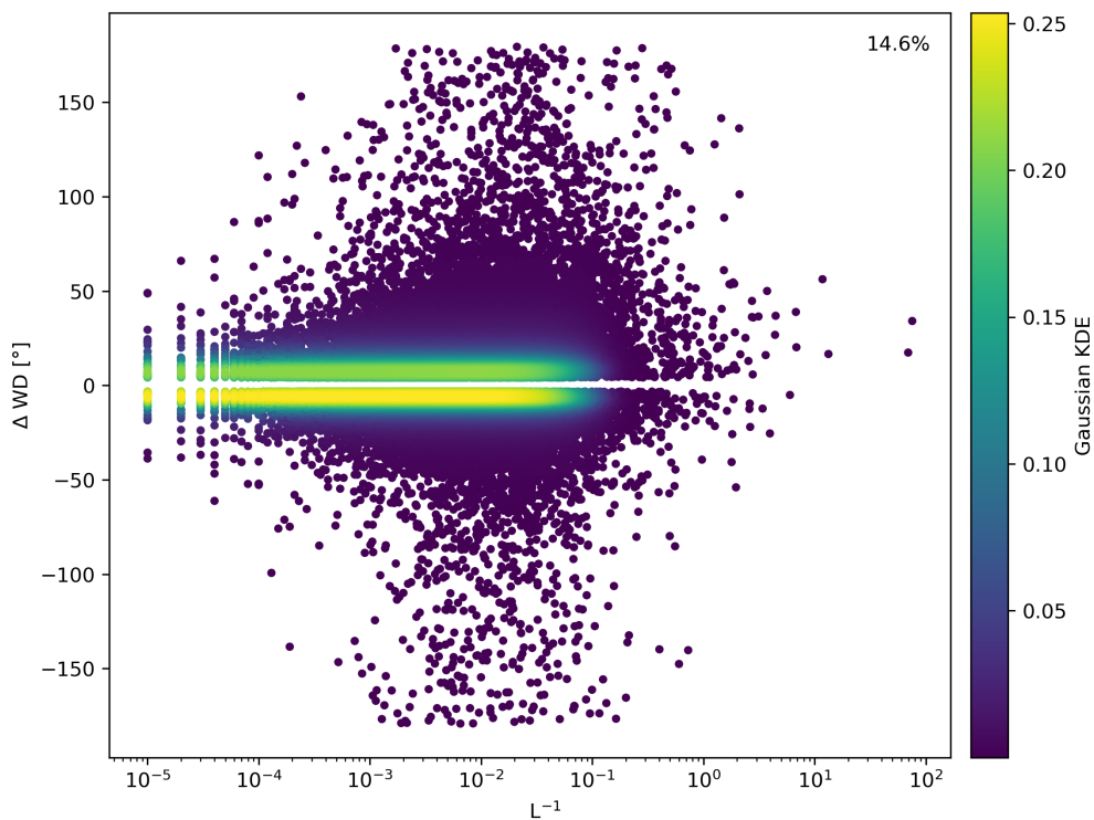
Figure 6. Wind direction difference ( \Delta WD ) at the inter-cluster scale (DBU - GT I) for neutral and stable atmospheric stratification. Only values for wind speeds above 2.5 \text{ ms}^{-1} and \Delta WD exceeding the lower and upper quartiles are shown, which results in 14.6 % of the data. The color shows a Gaussian Kernel density estimation (KDE).
