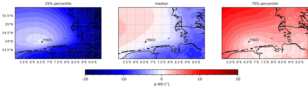
Figure 5. Wind-Statistics of local wind direction changes per 100 km with reference respect to FINO1 for the 30 years of NEWA data and different wind speed ranges. The left and right plots show the mean-of-the-annual-lower and upper quartiles respectively. The center plots shows the mean-of-show the yearly-medians-median for all wind speeds (upper row), the wind speed range 2.5 - 5.0 \text{ms}^{-1} (middle row) and 12.5 - 15.0 \text{ms}^{-1} (lower row). Note the different color scales for the wind speed ranges. The coastline and border data originate from the Natural Earth dataset (Natural-Earth, 2021) (Natural Earth, 2021).
