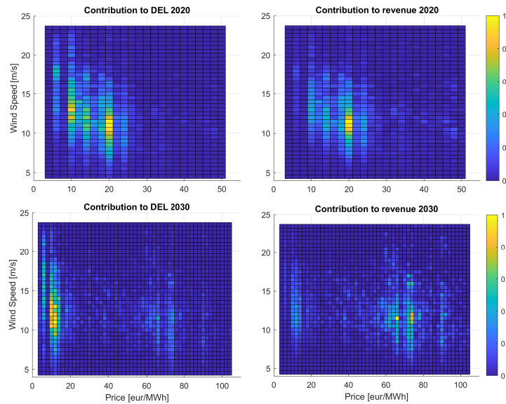
Figure 5. Contribution of price and wind speed bins to revenue and damage equivalent load (DEL) of blade root out-of-plane moment (BROop), obtained by multiplying the counts of each bin with the response obtained with the baseline wind turbine controller in simulations with the full datasets for 2020 and 2030. All values are normalised to the maximum value for the specific year and metric. Note that regions with high contributions to revenue on the right are strongly correlated to the bins with (below rated) wind speed and direction in Figure 1 included in the showcase with high day-ahead electricity prices.
