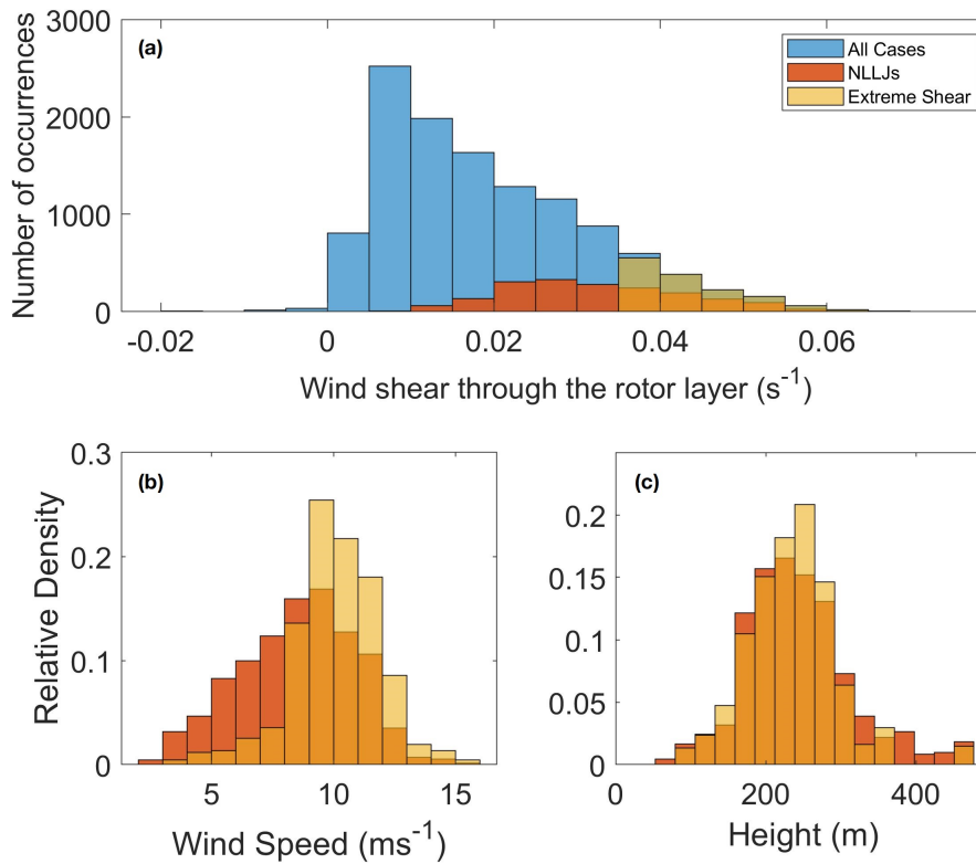
Figure 17. Vertical shear of wind speed in the rotor layer. Shown are (a) the number of occurrences of vertical shear in the rotor layer, and the frequency of (b) wind speed and (c) height. All conditions are shown in blue, NLLJs in red and extreme shear cases in yellow. Extreme shear was defined by the 90% percentile ( 0.0354 \text{ s}^{-1} )
