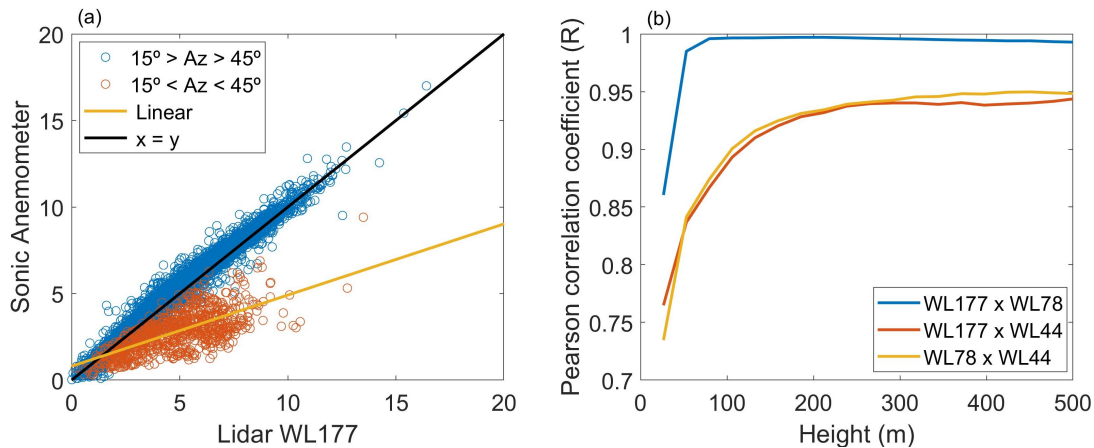
Figure 1. Data validation. Shown are (a) Comparison of the horizontal wind speed from the sonic anemometer against the LiDAR WL177, at about 90 m a.g.l. from. The comparison in the azimuth range between 15^\circ and 45^\circ is shown in red to highlight the sonic anemometer against effects of the LiDAR WL177, and tower shadowing effect. (b) the Pearson correlation coefficient (R) of the different LiDARs against the height a.g.l.. WL177 and WL78 are located in Falkenberg, while WL44 is operated \sim 6 km away in Lindenber.
