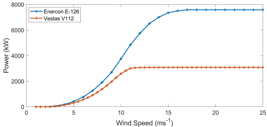
Figure 4. Power curves of the Enercon E-126 and Vestas V112 Onshore turbines. The E-126 turbine still produces energy until its cut-out wind speed of 34 \text{ ms}^{-1} .
