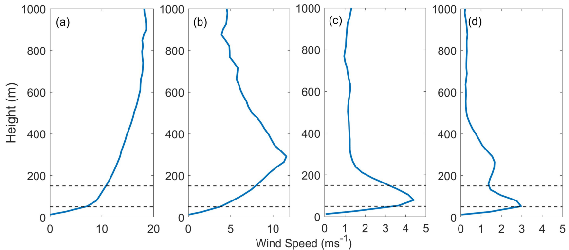
Figure 16. Examples of wind profiles with different vertical shears in the horizontal wind speed: (a) strong shear without the presence of a NLLJ, (b) strong shear due to a NLLJ, (c) a NLLJ with the core inside the rotor layer and (d) a NLLJ immediately below the rotor layer. The dashed lines mark the mean rotor layer of 50–150 m a.g.l..
