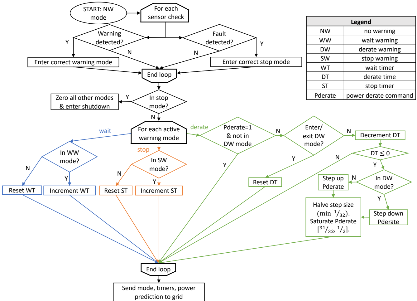
Figure 2. Warning logic flow diagram. Mode, timer, and predicted derate (logic not shown) are communicated to the grid. Predicted derate is meaningful once there is a derate warning, and is set to the derate value that will occur when the derate countdown hits zero. First, the controller checks for active warning modes. Then, for each warning mode active, the logic depends on the type of warning mode. If wait or stop, a timer is incremented to track how long it persists. Otherwise, it is reset. If derate, a countdown is started and decremented as long as the derate warning mode persists. If it reaches zero, the power command is halved. If the derate warning mode is exited, the controller seeks the highest power command it can operate at while staying below rated power and greater than or equal to \frac{1}{2} pu . The method is: If the derate countdown hits zero in derate warning mode, power decrements. If it hits zero out of derate warning mode, power increments, saturated to [\frac{1}{2}, \frac{31}{32}] pu . Steps are progressively halved in magnitude to seek the optimal power command.
