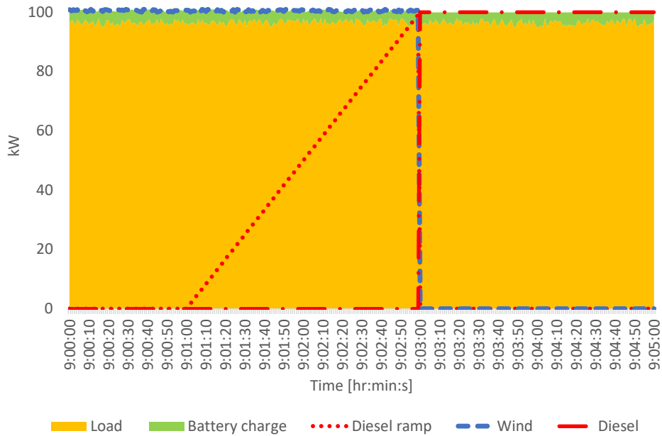
Figure 9. Scenario 2 baseline case. Abrupt wind turbine fault necessitates diesel emergency start and maximum battery discharge.
