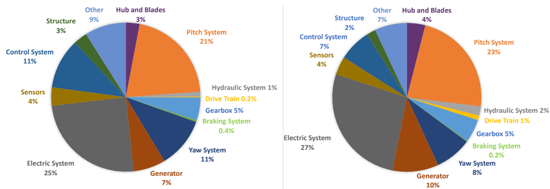
Figure 1. Failure rate (left) and downtime (right) as a result of various turbine subsystems. Figure generated from Reliawind report data (Wilkinson and Hassan, 2011).
