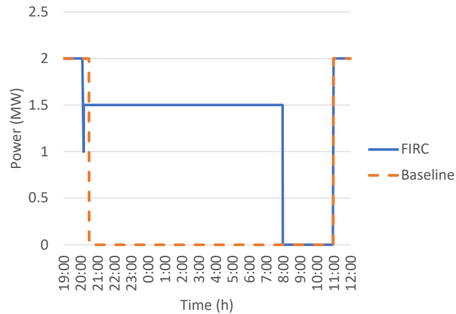
Figure 8. FIRC derates wind turbine to avoid fault, increasing wind power plant production by 17 MWh from time of high sensor readings to time of repair.
