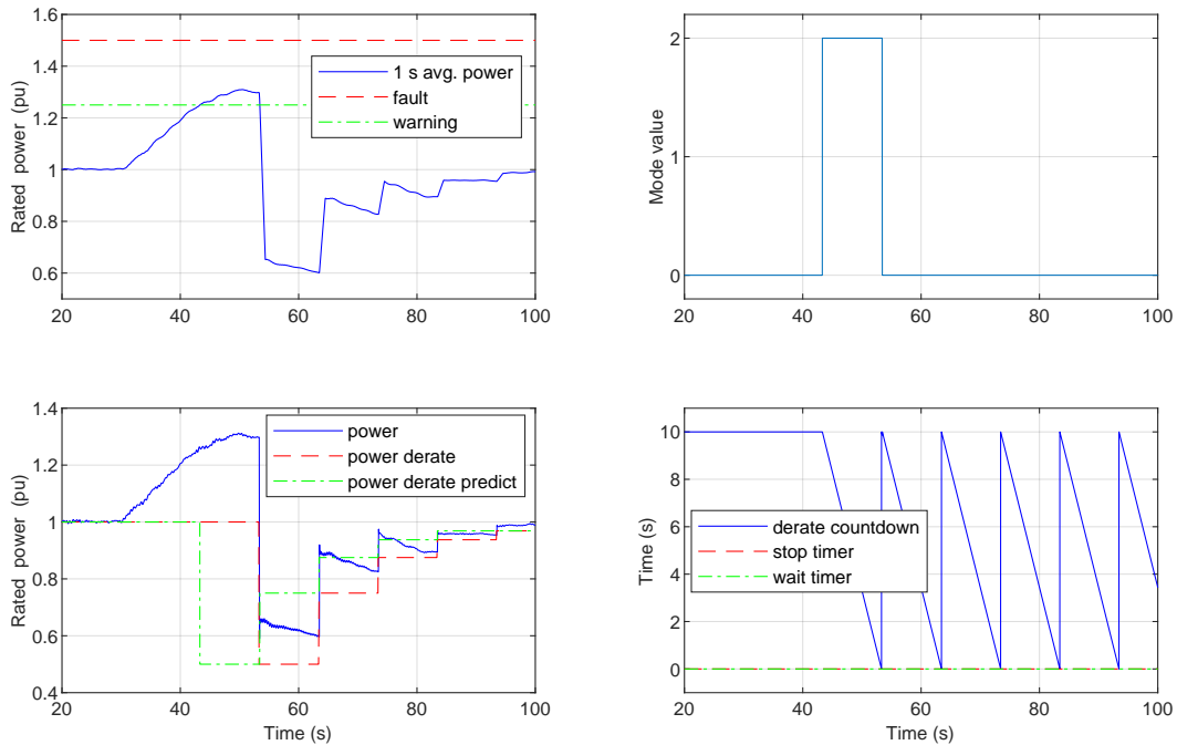
Figure 5. Case 1 scope. Overpower warning mitigated by derate. Power then progressively steps up to near 100% ( \frac{31}{32} pu ), with power staying below the warning threshold. Top left: 1 s avg. power signal with fault and warning thresholds. Bottom left: power prediction, command, and actual output. Top right: mode value, two=derate warning, zero=no warning. Bottom right: timers. In derate warning mode, derate countdown counts down from the user-defined max time. Each time it reaches zero, power command steps down if in derate warning mode or up if not in derate warning mode.
