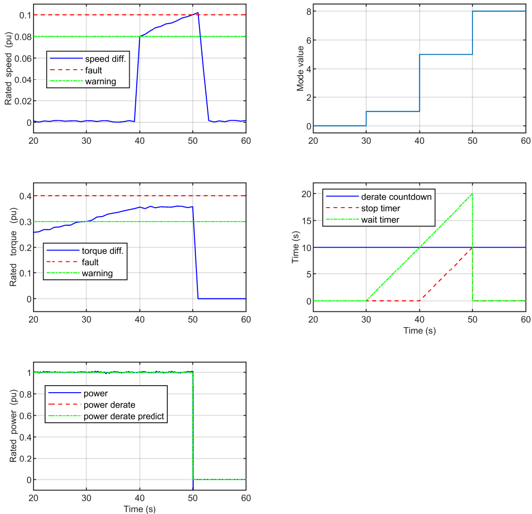
Figure 6. Case 2 scope. Speed sensor warning anticipates fault, which would give the grid operator time to react. Top left: HSS/LSS speed difference, with fault and warning thresholds. Mid left: HSS/LSS torque difference, with fault and warning thresholds. Bottom left: power prediction, command, and output. Top right: mode value. 0=no warning, 1=wait warning, 5=wait warning + stop warning, 8=normal stop. Mid right: timers. Stop and wait timers start counting up when stop and wait warning modes are activated, respectively, then reset when the wind turbine shuts down.
