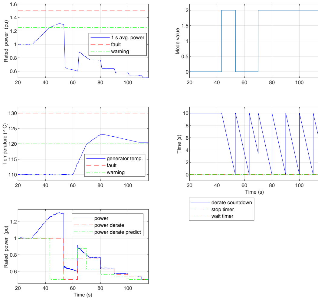
Figure 7. Case 3 scope. Interaction between two derate warnings. Derating mitigates the first warning, and the power command begins to step up, but the appearance of a second warning drives the power command to step back down. Top left: 1 second average power, with fault and warning thresholds. Mid left: generator temperature, with fault and warning thresholds. Bottom left: power prediction, command, and output. Top right: mode value. 0=no warning, 2=wait warning. Mid right: timers. In derate warning mode, derate countdown counts down from the user-defined max time. Each time it reaches zero, power command steps down if in derate warning mode or up if not. The timer resets when derate warning mode toggles on/off.
