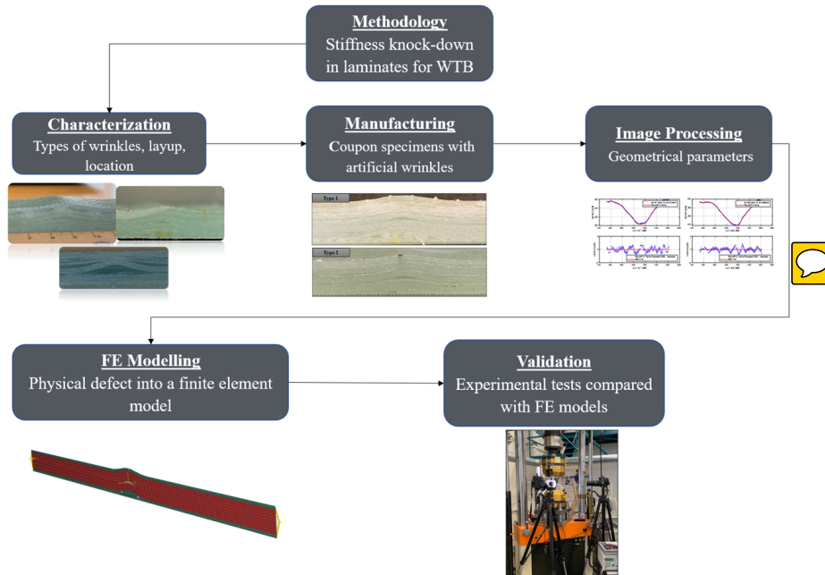
Figure 2. Schematic of the steps used to carry on the methodology of analysis to evaluate the stiffness knock-down of laminates for WTB.
