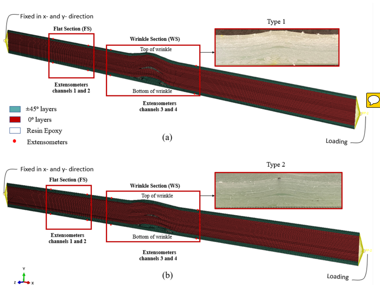
Figure 6. High fidelity finite element model modelled in a ply-by-ply sequence, with biaxial layers on top and bottom, UD layers in between and resin pocket around the biax fold and underneath the ply contour of max. amplitude : (a) coupon specimen model for wrinkle type 1 (b) coupon specimen model for wrinkle type 2.
