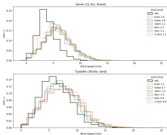
Figure 7. Probability density function (PDF) and Earth mover's distance (EMD) between simulations and measurements (OBS) for the various experiments in Table 1 and reanalyses, and two inland sites measured at lower heights.
