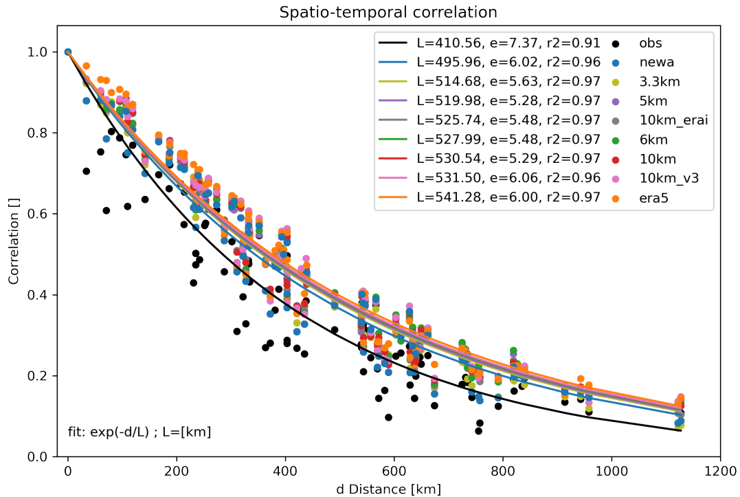
Figure 7. Correlation versus distance for each pair of sites (Table 2) and the fitted curves for the measurements (black) and the various model simulations in Table 1 and reanalyses. The estimated de-correlation length L is also shown for each simulation.
