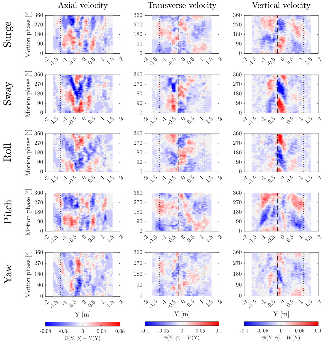
Figure 9. Space-time evolution of phase-averaged wake velocities ( \bar{u}(Y, \phi) axial, \bar{v}(Y, \phi) transverse, \bar{w}(Y, \phi) vertical, \phi is the motion phase): variation with respect to the mean velocity in each point ( U(Y) , V(Y) , W(Y) ). The results are obtained for motion at the wave frequency, for WC2, at X = 2.3D . The phase-averaging is done based on 94 motion cycles. The vertical dotted lines mark the edge of the rotor and the dashed vertical line is in correspondence of the average position of the wake center.
