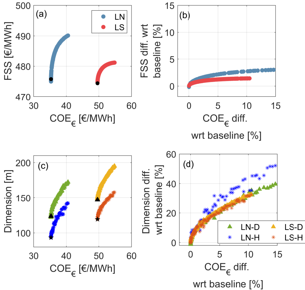
Figure 12. Pareto front between FSS and COE € , in absolute values (a), and relative to the COE € -driven baseline of each location (b). Optimal diameters and hub heights of the Pareto solutions in absolute values (c), and relative to the corresponding COE € -driven baseline of each location(d).
