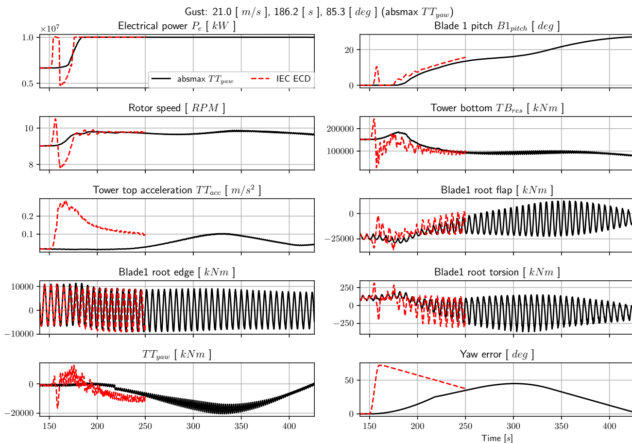
Figure A2. Gust for which the tower top yawing moment TT_{yaw} has the absolute maximum (see also table 2)
