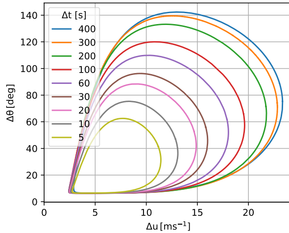
Figure 3. The 50-year return period surface, sliced at different rise times.
