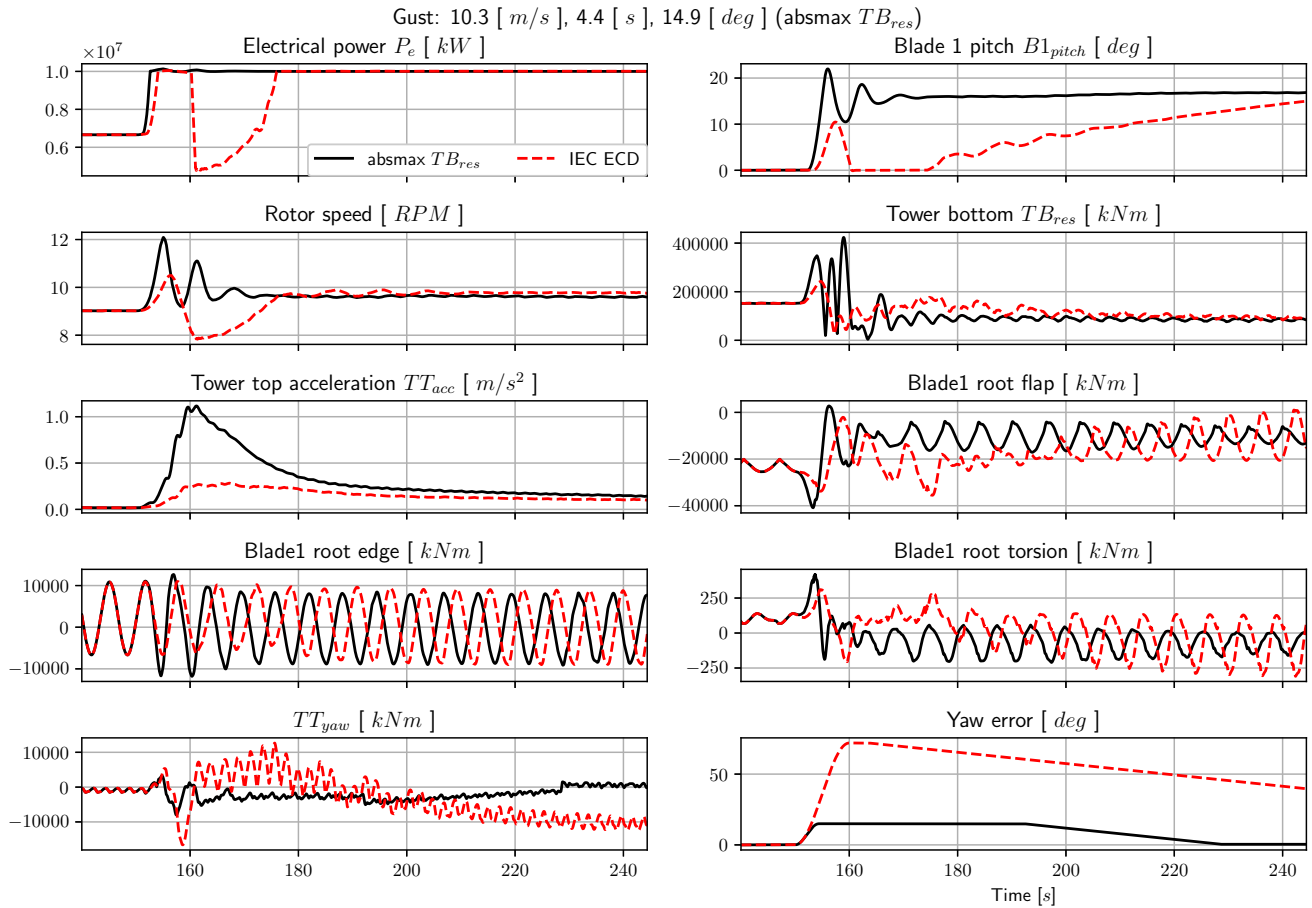
Figure A1. Gust for which the tower bottom resultant bending moment TB_{res} and the tower top acceleration TTabc has the absolute maximum (see also table 2)
