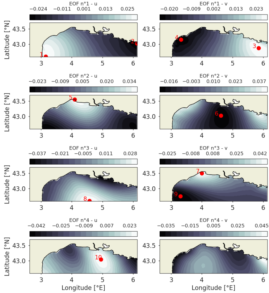
Figure 2. Selected sensors for the EOF extrema baseline in the Mediterranean Sea. The EOFs-EOF coefficients are displayed as background, and the selected salient points, and their associated ranks are displayed as red dots. The two columns are zonal ( u ) and meridional ( v ) wind speed, and the rows correspond to the EOF rank.
