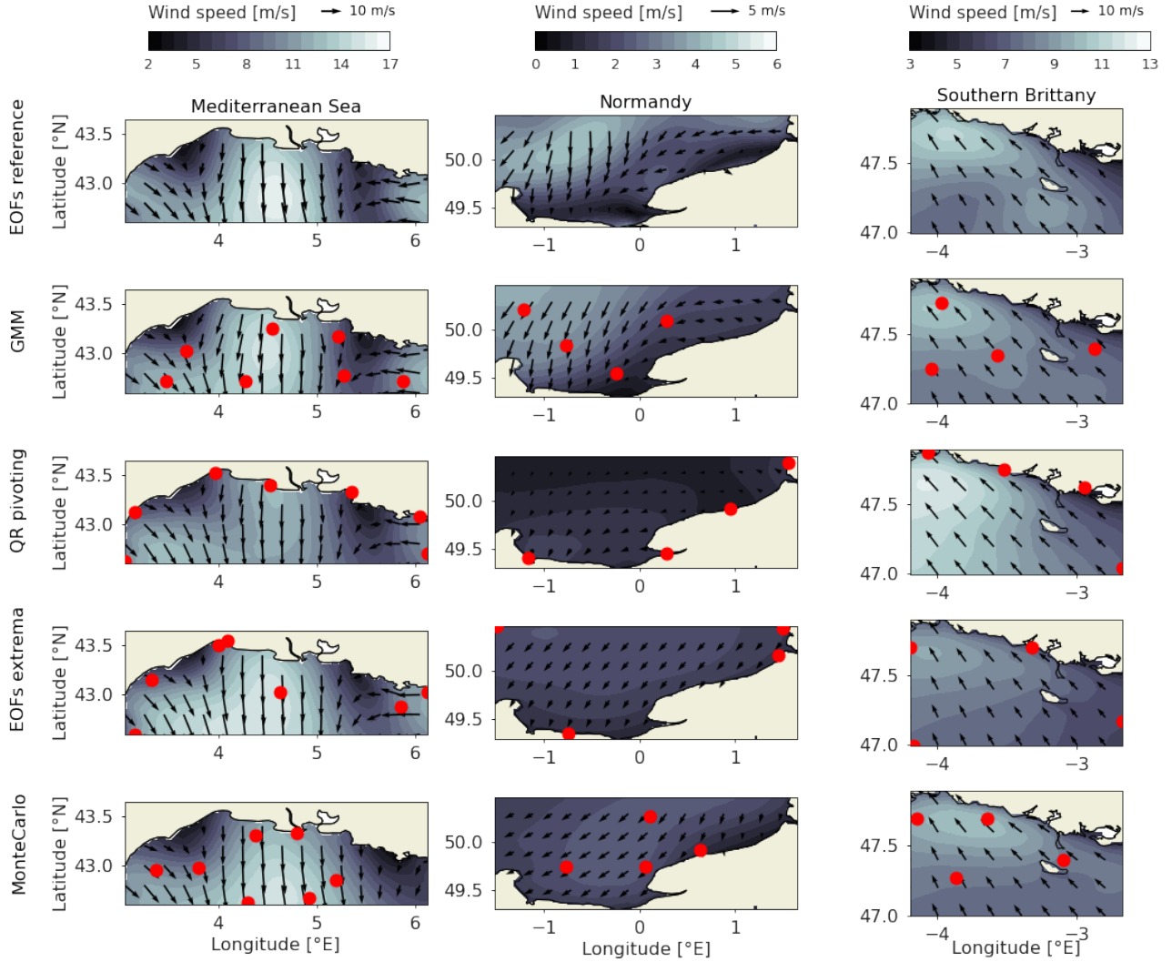
Figure 6. Reconstruction example for the optimal scenario on the three areas, from the reduced basis ( EOFs - EOF reference), from GMM clustering (GMM), and from the 3 baselines, QR pivoting, EOFs - EOF extrema and Monte Carlo. The color grading shows the wind speed, the black arrows the wind direction, with length proportional to the wind speed, and the red dots are the locations of the sensors on the optimal scenario, with 7 sensors on the Mediterranean Sea, and 4 for Normandy and Southern Brittany.
