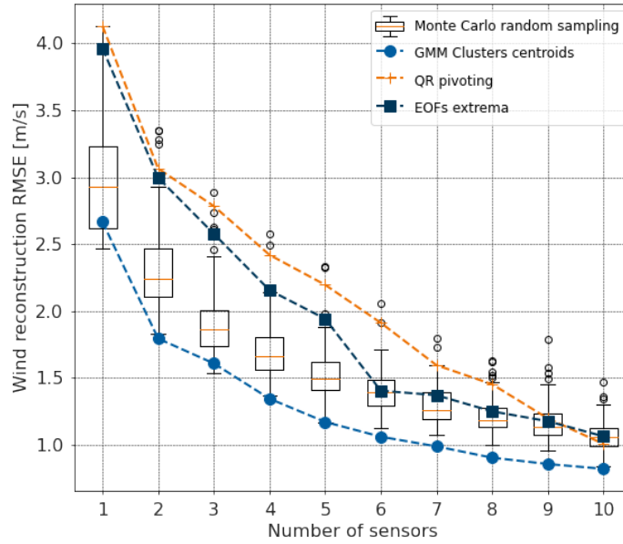
Figure 7. QR pivoting method (orange plus), EOFs-EOF extrema method (deep blue squares) and GMM method (blue dots) are compared to Monte Carlo simulations, displayed as boxplots in terms of wind reconstruction error.
