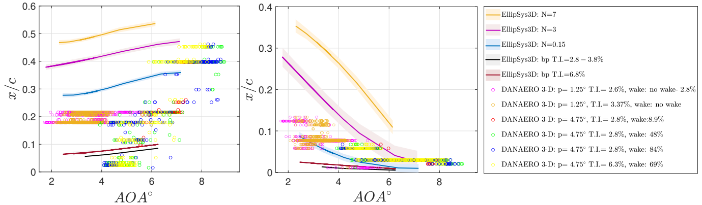
Figure 16. Detected transition locations from the EllipSys3D computations and the DAN-AERO field experiments for the pressure (left) and suction (right) sides, regrouped and regenerated from Özcakmak et al. (2020).
