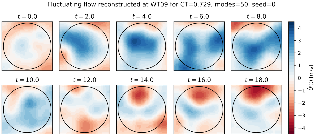
Figure 13. Instantaneous snapshots of the stochastic realizations of the streamwise velocity in a wake with C_T = 0.729 predicted with PS-ROM using 50 modes.
