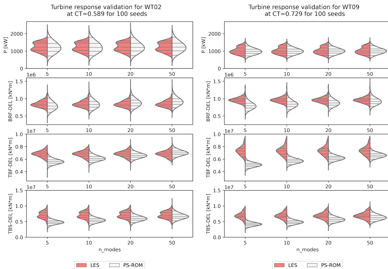
Figure 14. Distributions of 10min mean power and 1Hz damage equivalent load (DEL) of blade root flapwise (BRF), tower fore-aft (TBF), and tower side-side (TBS) bending moments for LES and for PS-ROM with 5, 10, 20, and 50 modes. Prediction at validation case, not used in the training of PS-ROM. Horizontal lines corresponds to 5, 25, 50, 75, and 95-percentiles. The statistics from PS-ROM is based on 100 random realizations of time series of 13, 107 [s] long corresponding to 2^{17} flow snapshots. WT02 is shown on the left and WT09 on the right.
