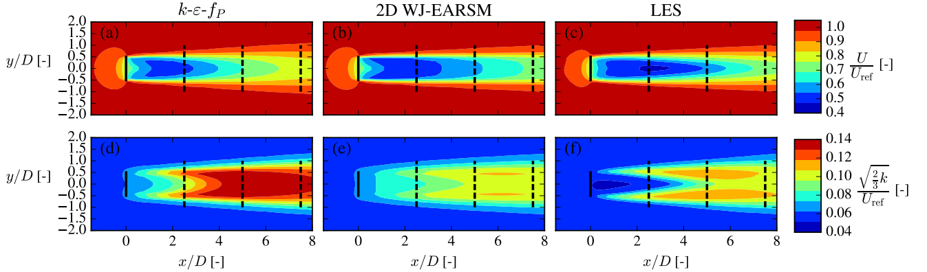
Figure 14. Streamwise velocity (upper row) and TI (lower row) contours at hub height for the single wake V80 case. Full lines mark ADs, while dashed lines mark where wake profiles are extracted.
