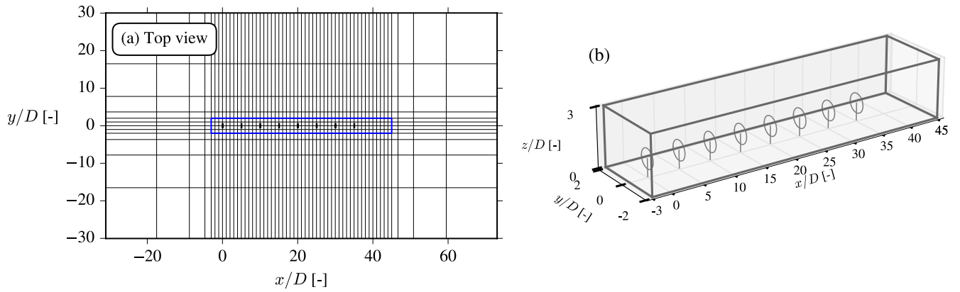
Figure 20. A xy-cut of the domain with every eighth cell shown (a) and a 3D view of the wake domain (b) for the aligned row case. The size of the domain is L_x/D = 104 , L_y/D = 60 and L_z/D = 25 . A rough wall BC and an inlet BC are used for the lower and upper BCs, respectively.
