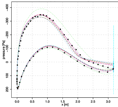
(c) Pressure at r=13.12 m
