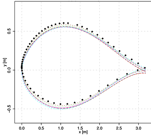
(a) Sectional geometry at r=13.12 m
