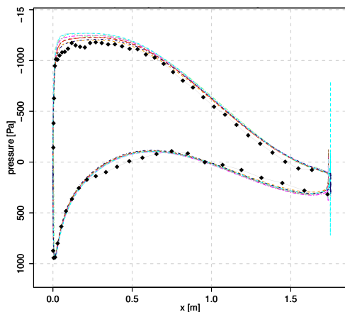
(e) Pressure at r=30.20 m
