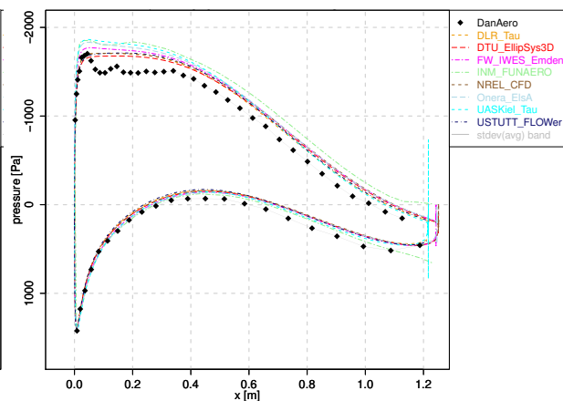
(f) Pressure at r=36.78 m
