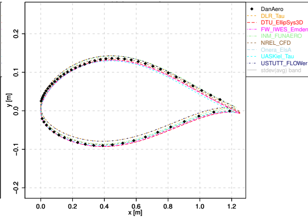
(b) Sectional geometry at r=36.78 m
