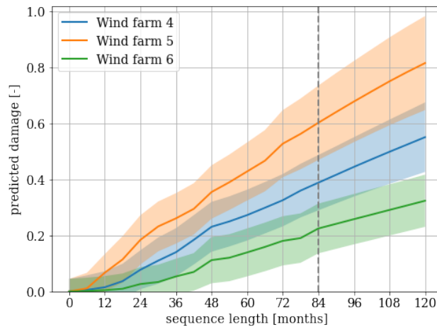
Figure 15. Example of the predicted damage progression for three different wind farms for varying sequence lengths and zero initial damage. Each sequence begins on 01-01-2013.
