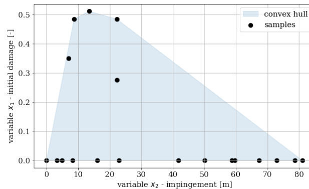
Figure 10. Visualization of the two-dimensional input variable space covered by the available training data and the corresponding convex hull.
