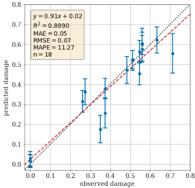
Figure 12. One-to-one comparison of ensemble predictions and the true observed damage (both encoded). The error bars indicate the ensemble standard deviation, the red dashed line shows the best linear fit, and the black dotted line shows the results of a perfect prediction as a reference.
