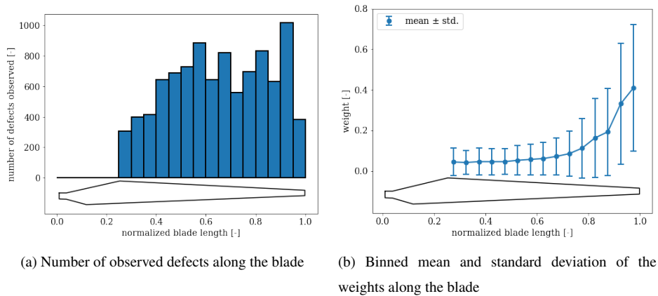
Figure 7. The total number of defects observed per cross-section of the blade (left), and the corresponding defect weights (mean and standard deviation, right).
