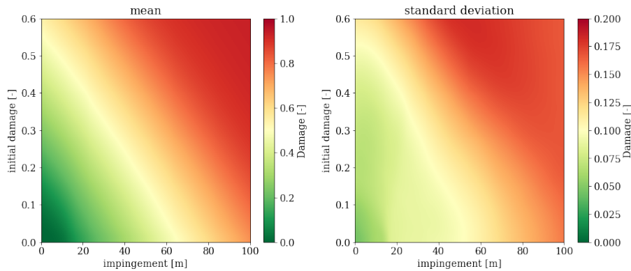
Figure 14. Color maps used as physics checks to validate the ensemble model response across the two-dimensional input space. The left figure shows the ensemble mean and the right figure shows the ensemble standard deviation.
