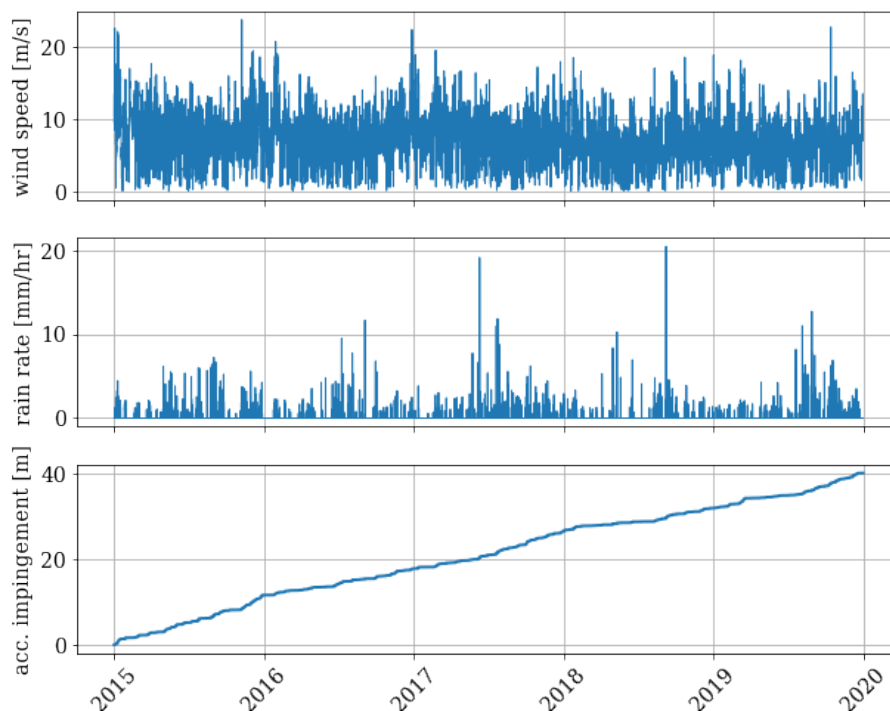
Figure 4. Example of a 5-year time series of wind speed (top), rain (middle), and accumulated rain impingement (bottom) from one of the training sites.
