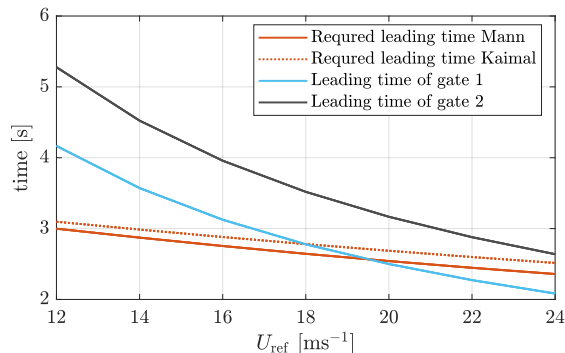
Figure 8. The leading time and required leading time for pitch forward command feedforward signal .
