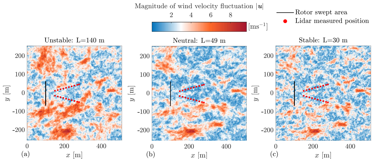
Figure 1. Top view of a turbulence field showing the eddy structures under different atmospheric stability, simulated using the 4D-Mann turbulence generator 4D Mann Turbulence Generator with parameters listed in Table 1. The lidar measured positions are plotted based on a typical four-beam pulse-pulsed lidar. The rotor swept-area swept-area is drawn based on the NREL 5.0 MW reference wind turbine which has a rotor diameter of 126 m. The length scales L are chosen based on studies by Peña (2019) and Guo et al. (2022a).
