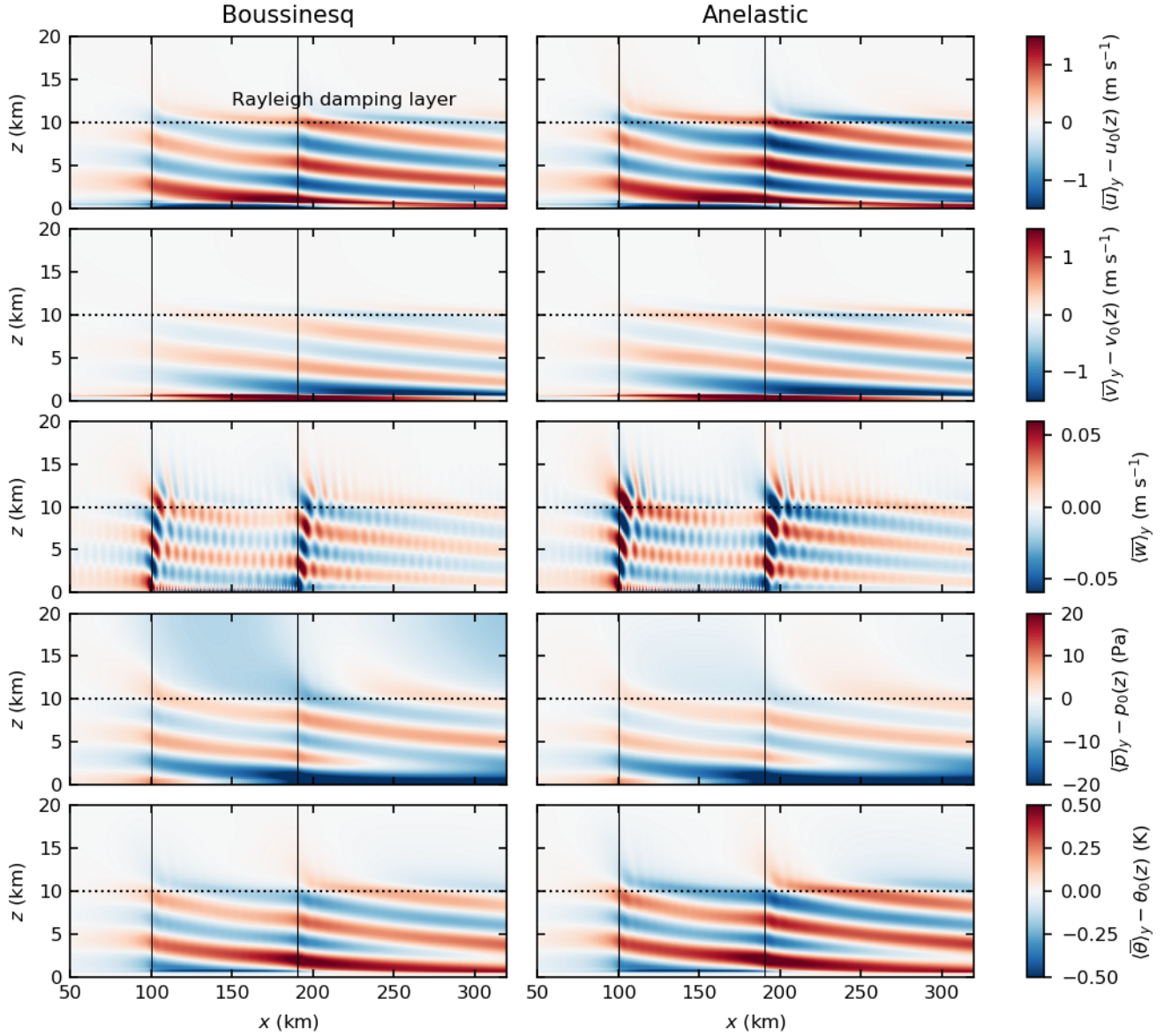
Figure A1. Wave fields for the test simulation with Boussinesq approximation approximation (left) and anelastic approximation (right). All quantities are averaged in time and along y and are given as deviations to the inflow profile.
