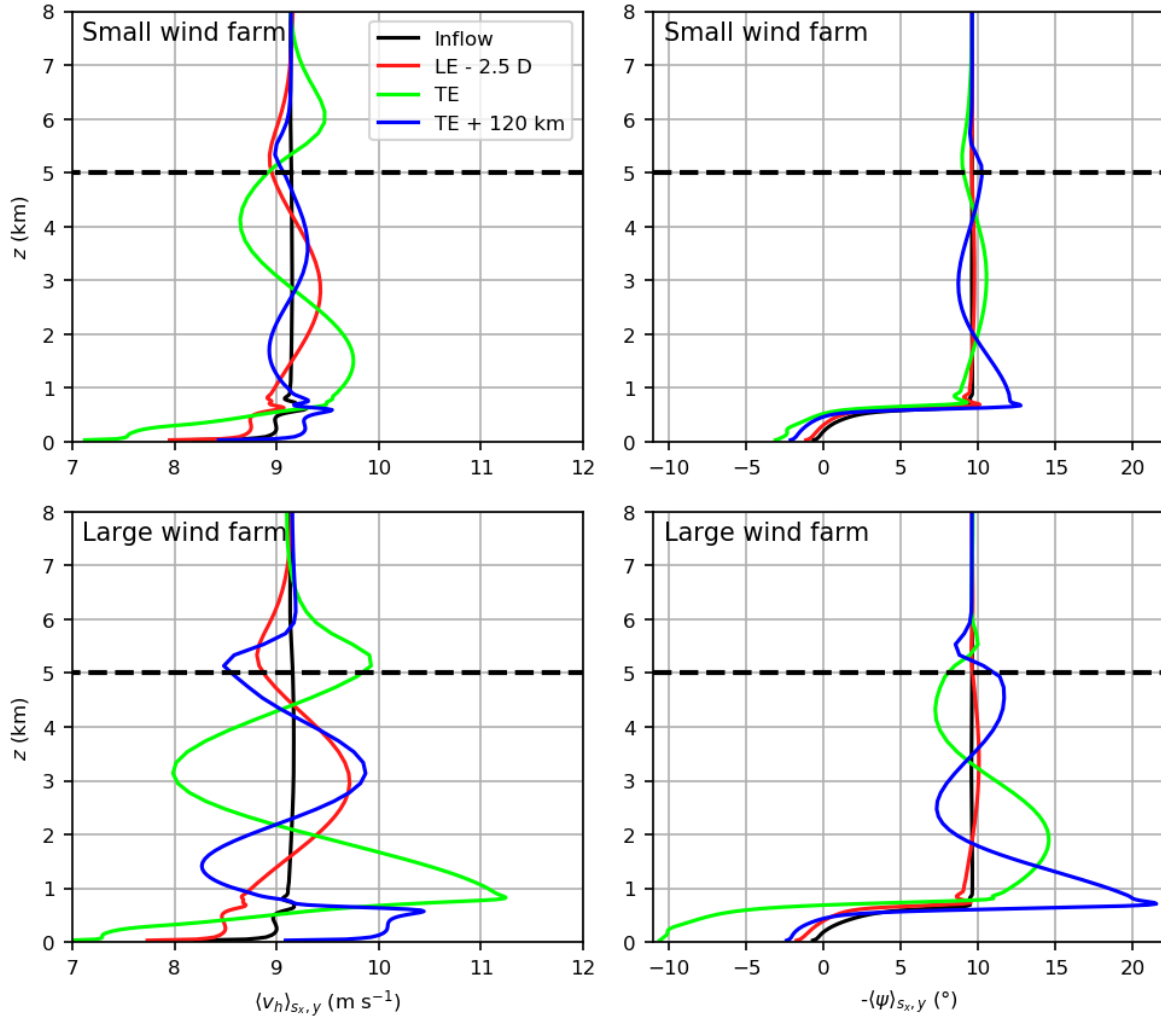
Figure 10. Vertical profiles of the horizontal wind speed (left) and the wind direction (right) for the small wind farm (top) and the large wind farm (bottom). The profiles are averaged in time, along y and over one turbine spacing along x . Horizontal dashed line indicates the bottom of the Rayleigh damping layer.
