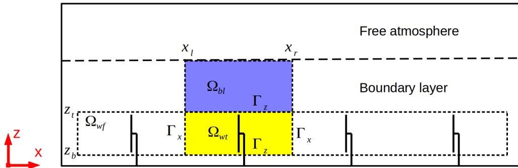
Figure 11. Sketch of wind turbine control volumes \Omega_{wt} , BL control volumes \Omega_{bl} and the wind farm control volume \Omega_{wf} . In x -direction the control volumes are bounded by the surfaces \Gamma_x at x = x_l and x = x_r . In the vertical direction, the control volumes are bounded by \Gamma_z at z = z_b and z = z_t . In y -direction the control volumes are bounded by the cyclic domain boundaries. The control volumes are centered on the respective turbine hub.
