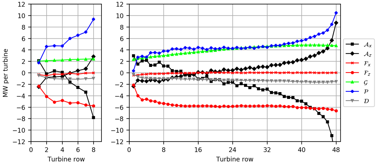
Figure 14. Energy budgets inside the BL control volumes \Omega_{bl} for the small wind farm (left) and the large wind farm (right). The budget terms are: horizontal advection of KE ( \mathcal{A}_x ), vertical advection of KE ( \mathcal{A}_z ), turbulent fluxes through left/right ( \mathcal{F}_x ) and bottom/top ( \mathcal{F}_z ) surfaces, geostrophic forcing ( \mathcal{G} ), perturbation pressure gradients ( \mathcal{P} ) and dissipation ( \mathcal{D} ). The buoyancy term ( \mathcal{B} ) is not shown, because it is very small. There is no energy extraction by wind turbines ( \mathcal{W} ) in the BL control volume.
