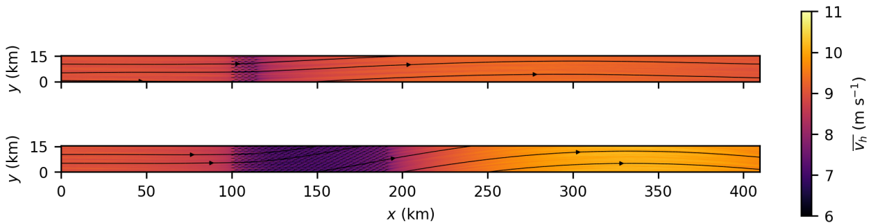
Figure 2. Mean horizontal wind speed at hub height for the small wind farm (top) and large wind farm (bottom). Wind direction is indicated by streamlines.
