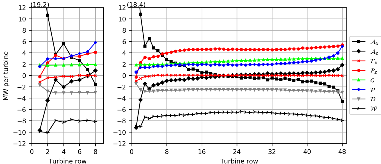
Figure 13. Energy budgets inside the wind turbine control volumes \Omega_{wt} for the small wind farm (left) and the large wind farm (right). The budget terms are: horizontal advection of KE ( \mathcal{A}_x ), vertical advection of KE ( \mathcal{A}_z ), turbulent fluxes through left/right ( \mathcal{F}_x ) and bottom/top ( \mathcal{F}_z ) surfaces, geostrophic forcing ( \mathcal{G} ), perturbation pressure gradients ( \mathcal{P} ), dissipation ( \mathcal{D} ) and wind turbines ( \mathcal{W} ). The buoyancy term ( \mathcal{B} ) is not shown, because it is very small.
