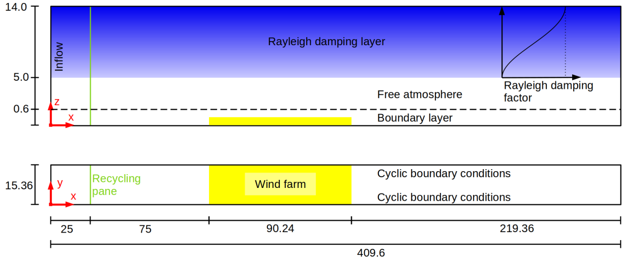
Figure 1. Side view and plan view of the domain and wind farm layout for the large wind farm case. Dimensions in km.
