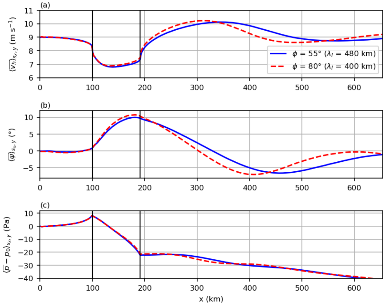
Figure B1. Horizontal wind speed, wind direction and relative perturbation pressure at hub height for the large wind farm case and a latitude of \phi = 55^\circ and \phi = 80^\circ .
