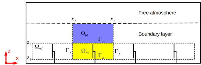
Figure 11. Sketch of wind turbine control volumes \Omega_{\text{wt}} , BL control volumes \Omega_{\text{bl}} and the wind farm control volume \Omega_{\text{wf}} . In the x direction the control volumes are bounded by the surfaces \Gamma_x at x = x_l and x = x_r . In the vertical direction, the control volumes are bounded by \Gamma_z at z = z_b and z = z_t . In the y direction the control volumes are bounded by the cyclic domain boundaries. The control volumes are centered on the respective turbine hub.
