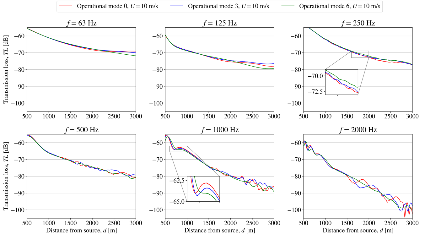
Figure 5. Setup 1: The transmission loss, TL , obtained from WindSTAR computations from a single SWT-DD-142 wind turbine subject to changing operational modes at each octave band frequency at a free field wind speed of U_{hub} = 10 \text{ m s}^{-1} at hub height.
