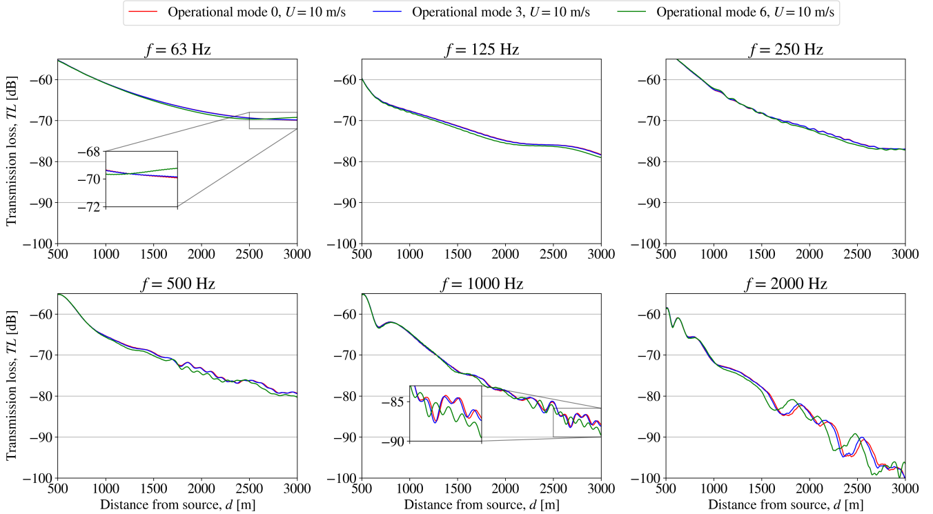
Figure 6. Setup 2: The transmission loss, TL , obtained from WindSTAR computations from a single SWT-DD-142 wind turbine positioned in the wake of a wind turbine subject to changing operational modes at each octave band frequency at a free field wind speed of U_{hub} = 10 m s -1 at hub height.
