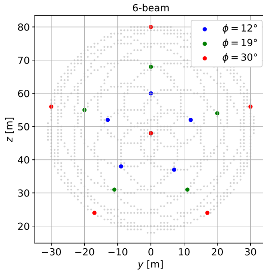
Figure 9. Selected grid cells for the 6-beam lidar with three different levels of the half-cone opening angle. The central grid coincides in the three cases. The gridded SpinnerLidar scans are shown in light grey.
