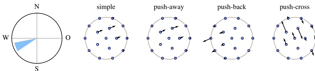
Figure 8. Pseudo-gradient vectors associated with a single wind direction for the IEA Wind Task 37 Case Study-case study 1 initial layout. (Reproduced from Quaeghebeur et al., 2021, which contains further details.)
