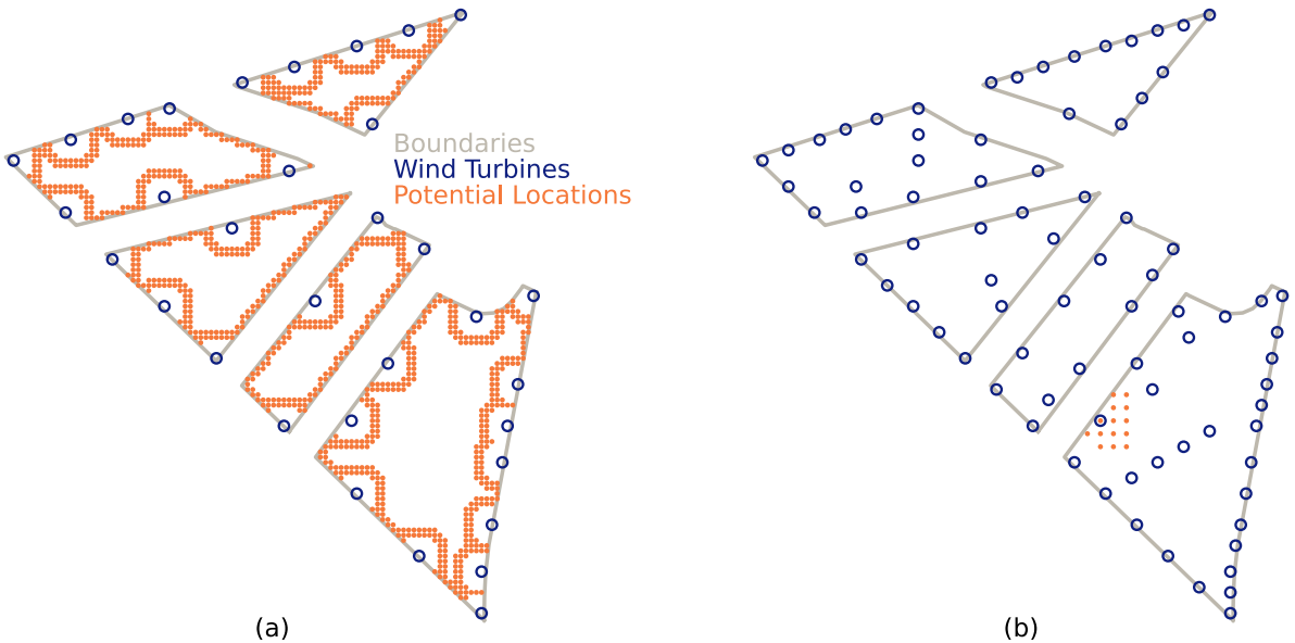
Figure 5. Visualization of the two phases of the DEBO algorithm. (a) An iteration of the greedy part of the DEBO algorithm. Potential locations are candidates for the next turbine’s location. (b) An Part of an iteration of the local-search part-portion of the DEBO algorithm for refining the position of one turbine. Potential locations are the discrete neighborhood of the turbine to be moved. Labels in (a) also apply to (b). Turbine markers are to scale with diameter equal to the turbine rotor diameter.
