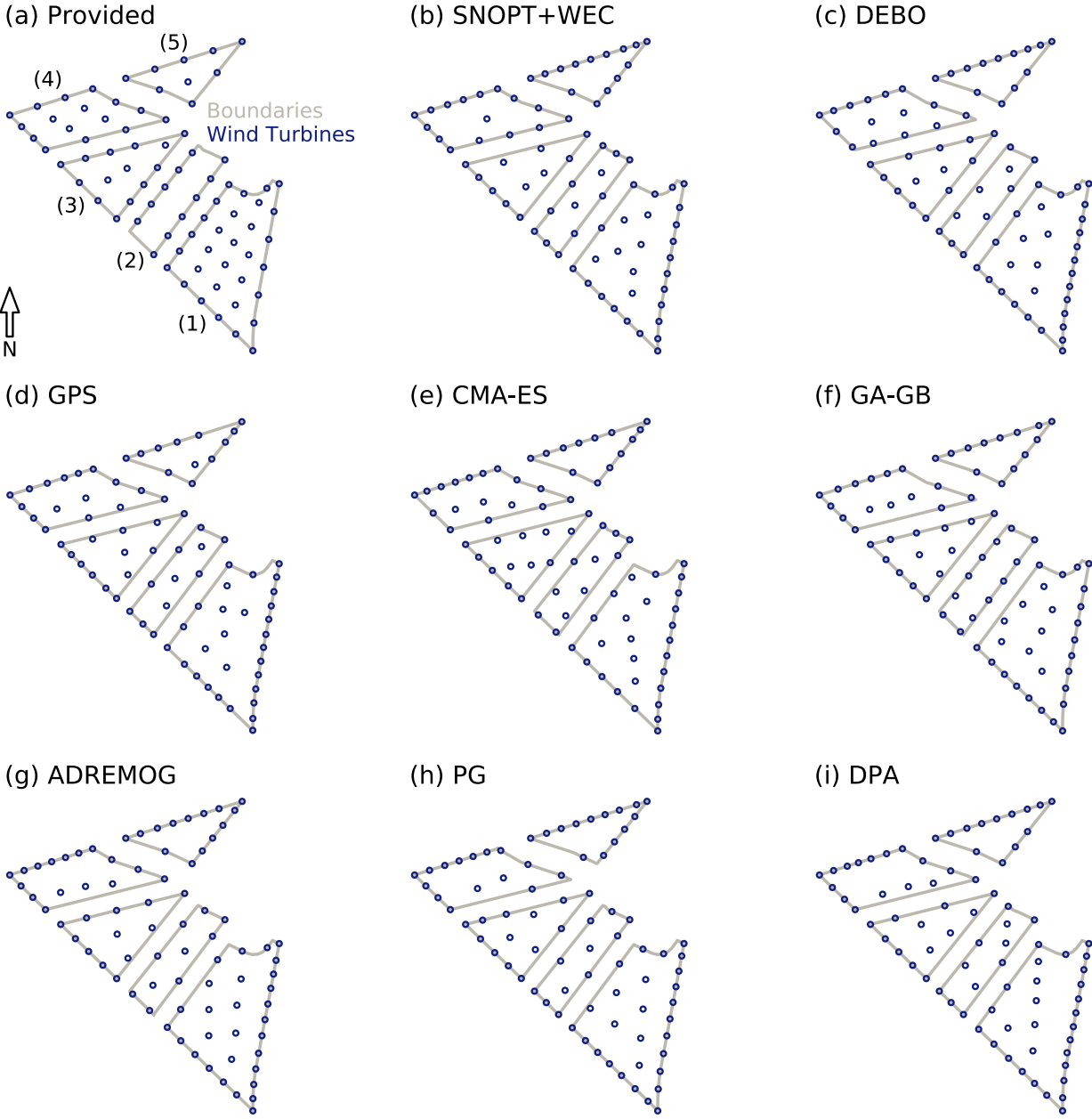
Figure 10. Best layout found for each algorithm. Labels in (a) also apply to (b) to (i).
