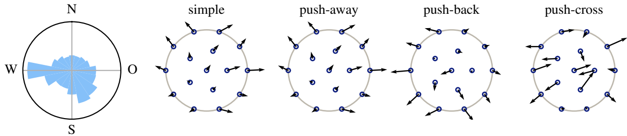
Figure 9. Pseudo-gradient vectors for the IEA Wind Task 37 Case Study - case study 1 initial layout and wind rose. (Reproduced from Quaeghebeur et al., 2021, which contains further details.)
