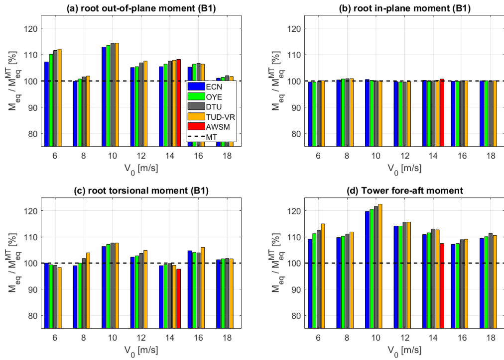
Fig. 4: same as figure 10 in the paper but including the AWSM simulation with prescribed pitch & rpm at 14m/s.
