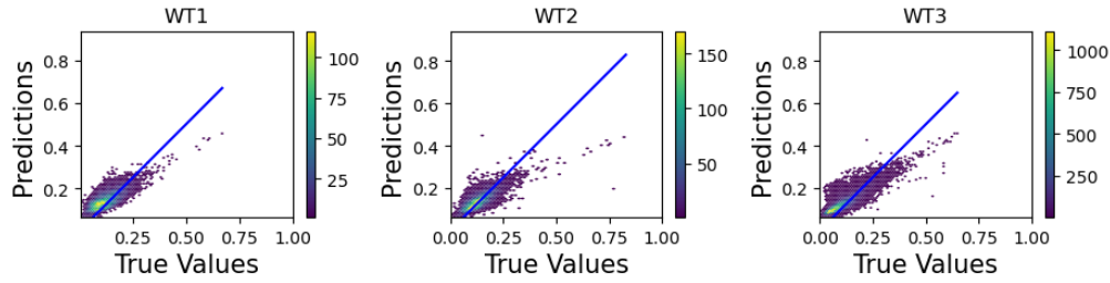
Figure 6. Error plot showing the predictions from the general model against the actual value for the DEM 2 of all three WTGs.
