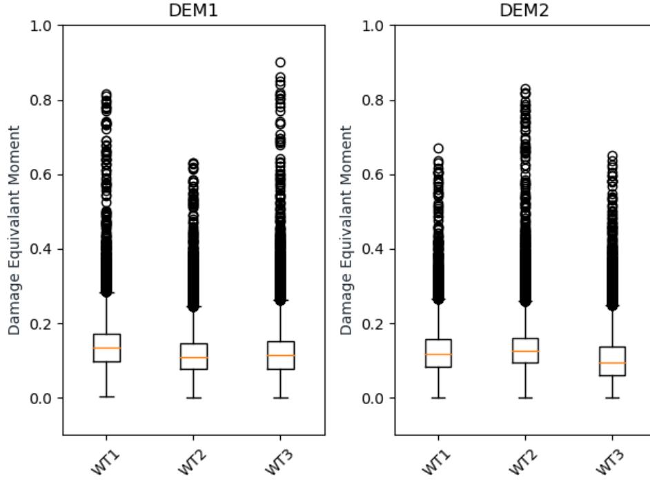
Figure 2. Normalised damage equivalent moments box plot of the two orthogonal directions for all three of the wind turbines.
