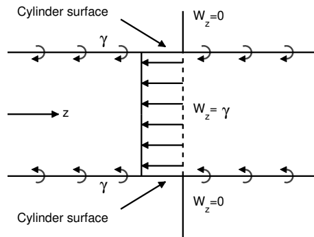
Figure 2. Sketch of velocity field induced by an infinite cylinder of tangential vorticity \gamma
