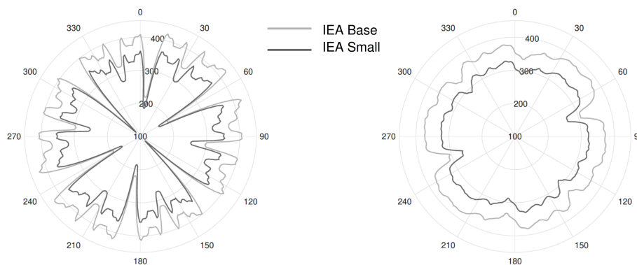
Figure 8. Power output in MW as a function of wind direction for the (a) Regular and (b) Irregular wind farm layout with the IEA Base (light-grey) and IEA Small (dark-grey) turbines, with a mean wind speed of 9.5 m/s (Sickler, 2020).
