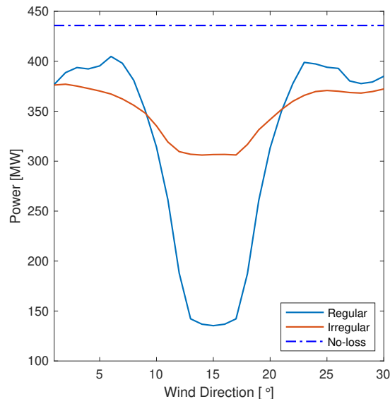
Figure 5. Power output of wind farms with regular and irregular layouts at a wind speed of 9.5 m/s as functions of wind direction, zoomed in on the wind directions with the largest power drops (Sickler, 2020).
