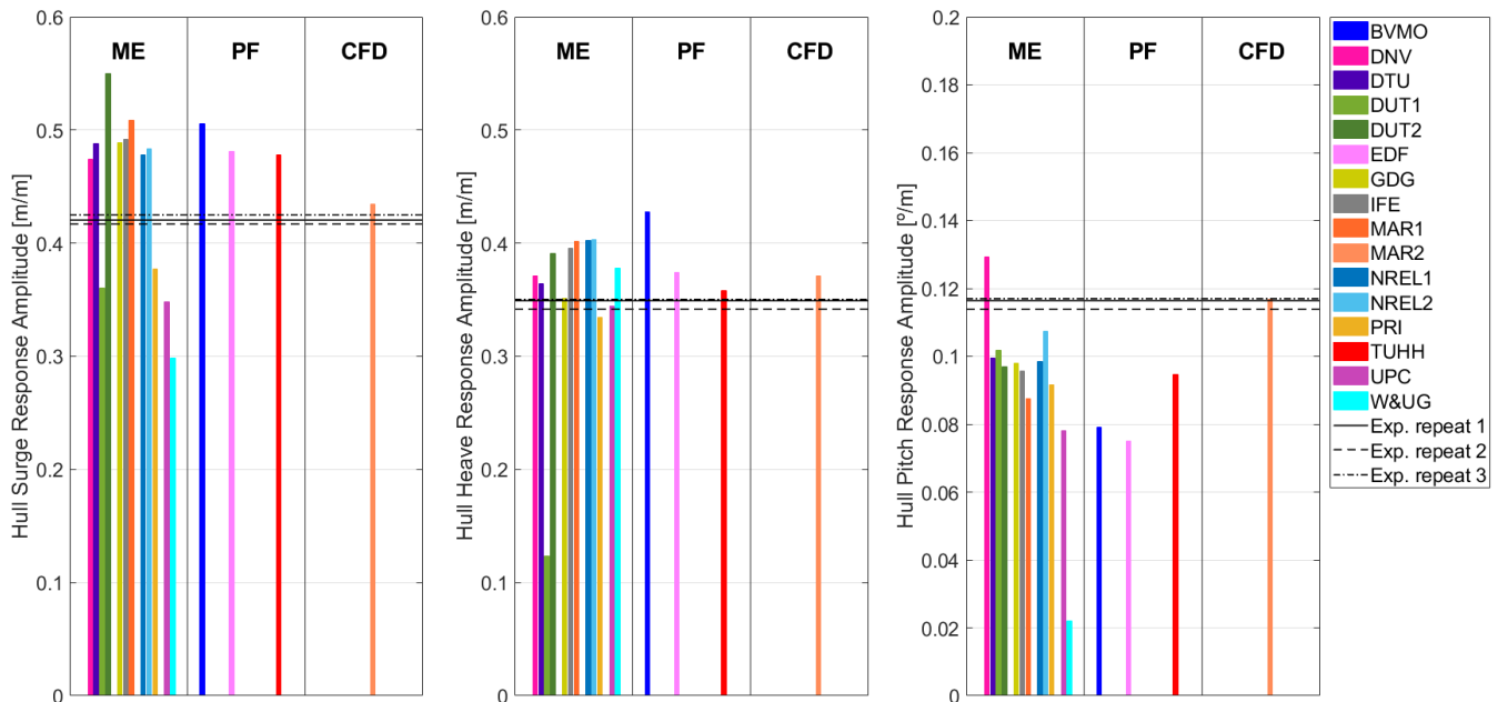
455 Figure 5: Normalized response amplitude at the wave frequency in Load Case 4.1 for the surge, heave, and pitch degrees of freedom. Outputs sorted out according to the hydrodynamic theory: Morison equation (ME), potential flow (PF) augmented with viscous drag, and computational fluid dynamics (CFD).
