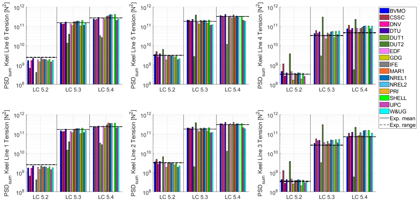
Figure 19: Power spectral density (PSD) sum of the six keel lines for the combined wind and wave conditions in Load Cases (LC) 5.2, 5.3, and 5.4. Vertical axis in logarithmic scale.
