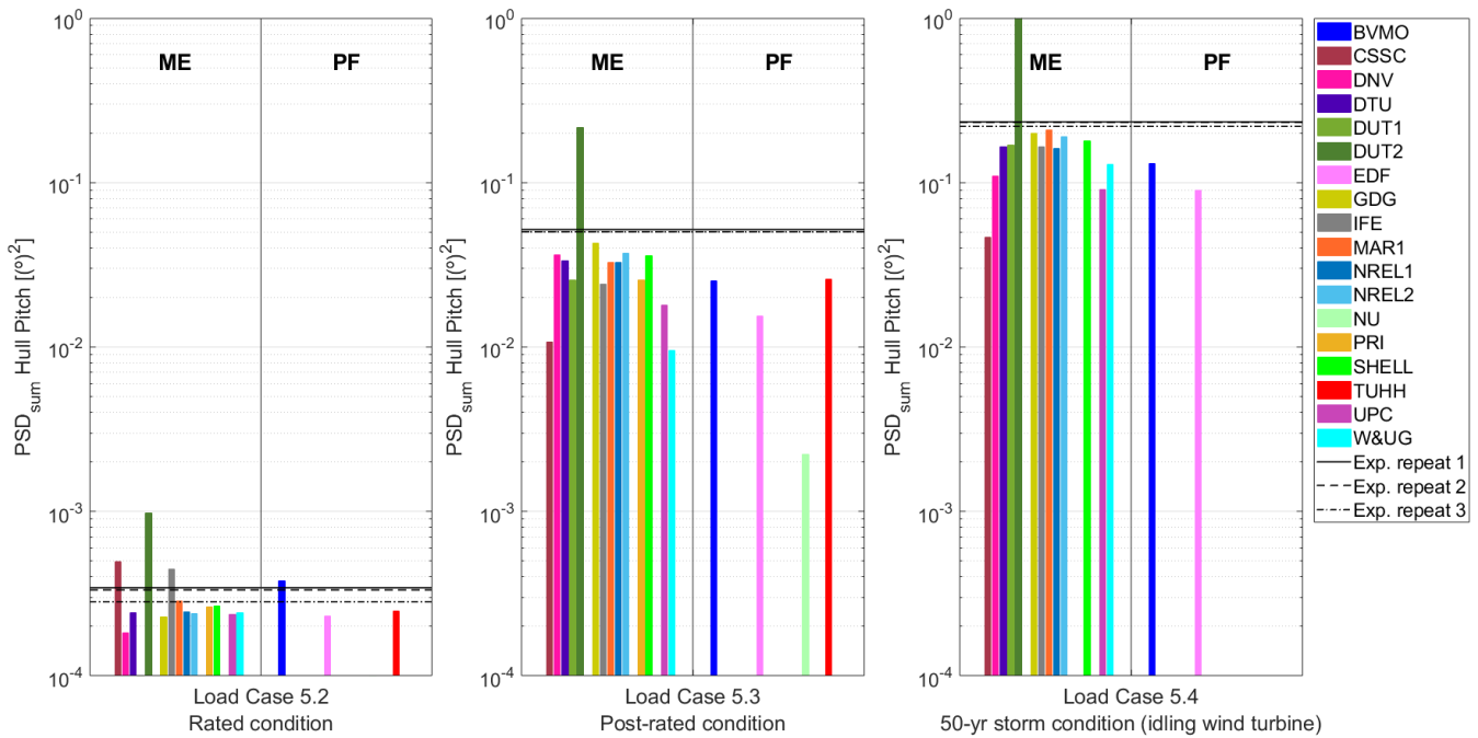
510 Figure 9: Power spectral density (PSD) sum of the hull pitch motion for the combined wind and wave conditions in Load Cases 5.2, 5.3, and 5.4. Outputs sorted out according to the hydrodynamic theory: Morison equation (ME) and potential flow (PF). Vertical axis in logarithmic scale.
