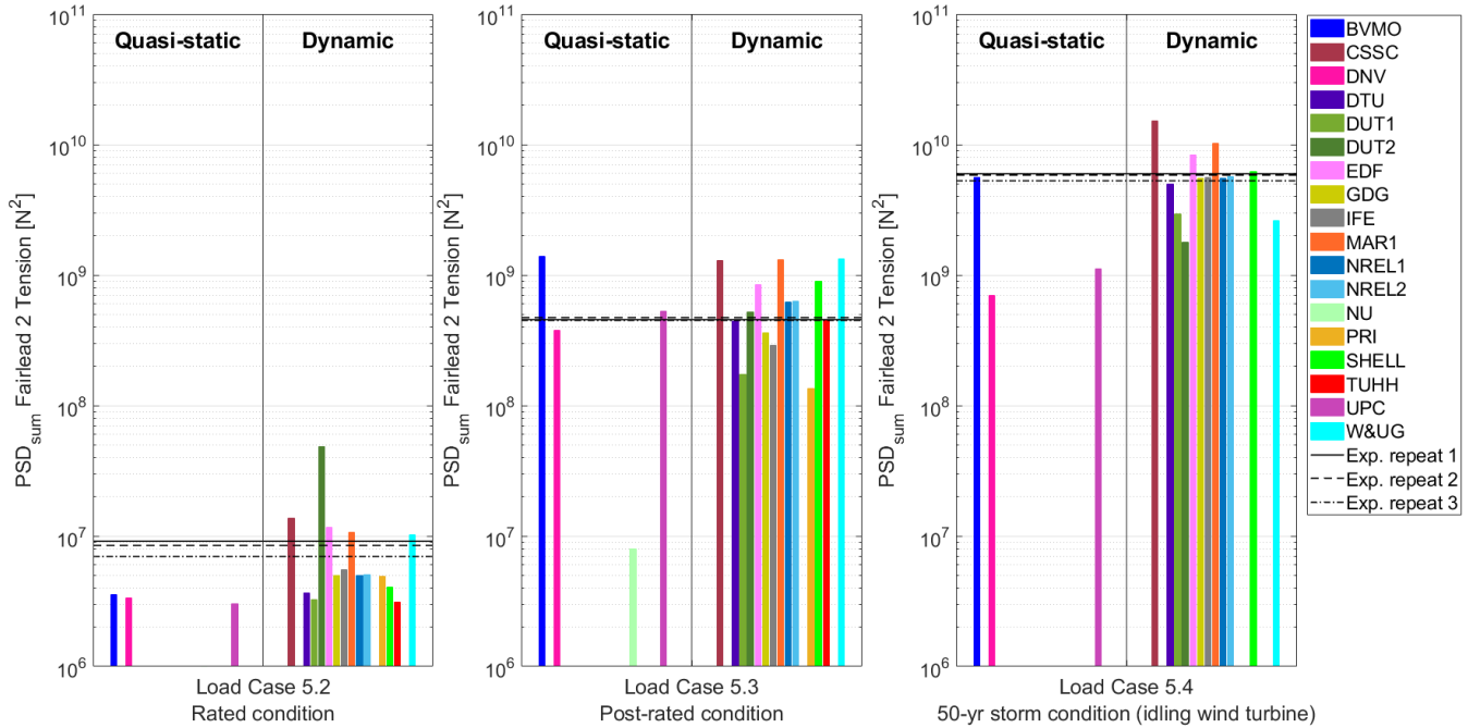
Figure 15: Power spectral density (PSD) sum of the fairlead 2 tension for the combined wind and wave conditions in Load Cases 5.2, 5.3, and 5.4. Outputs sorted out according to the mooring line theory: quasi-static and dynamic. Vertical axis in logarithmic scale.
