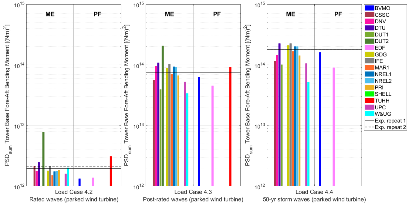
Figure 11: Power spectral density (PSD) sum of the fore-aft tower base bending moment for the wave-only conditions in Load Cases 4.2, 4.3, and 4.4. Outputs sorted out according to the hydrodynamic theory: Morison equation (ME) and potential flow (PF) with augmented viscous drag. Vertical axis in logarithmic scale.
