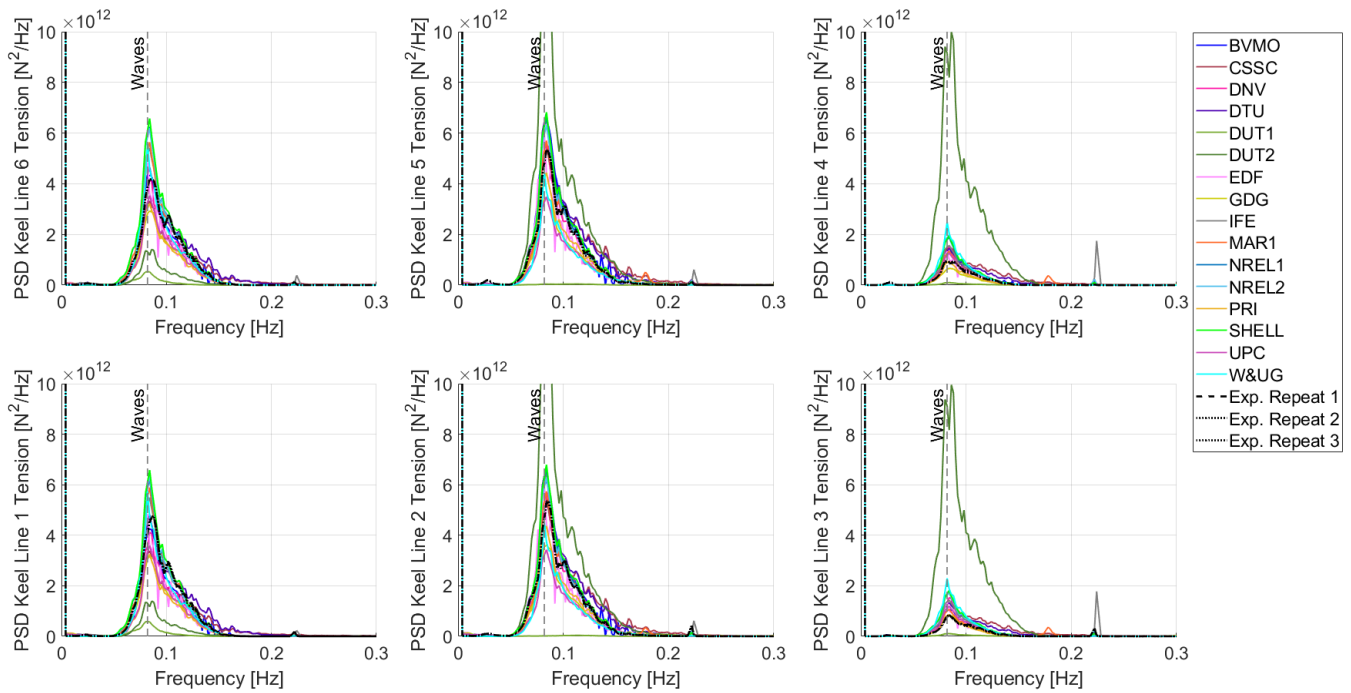
690 Figure 18: Power spectral density (PSD) for the six keel lines in the combined wind and wave conditions for the post-rated operating condition (Load Case 5.3).
