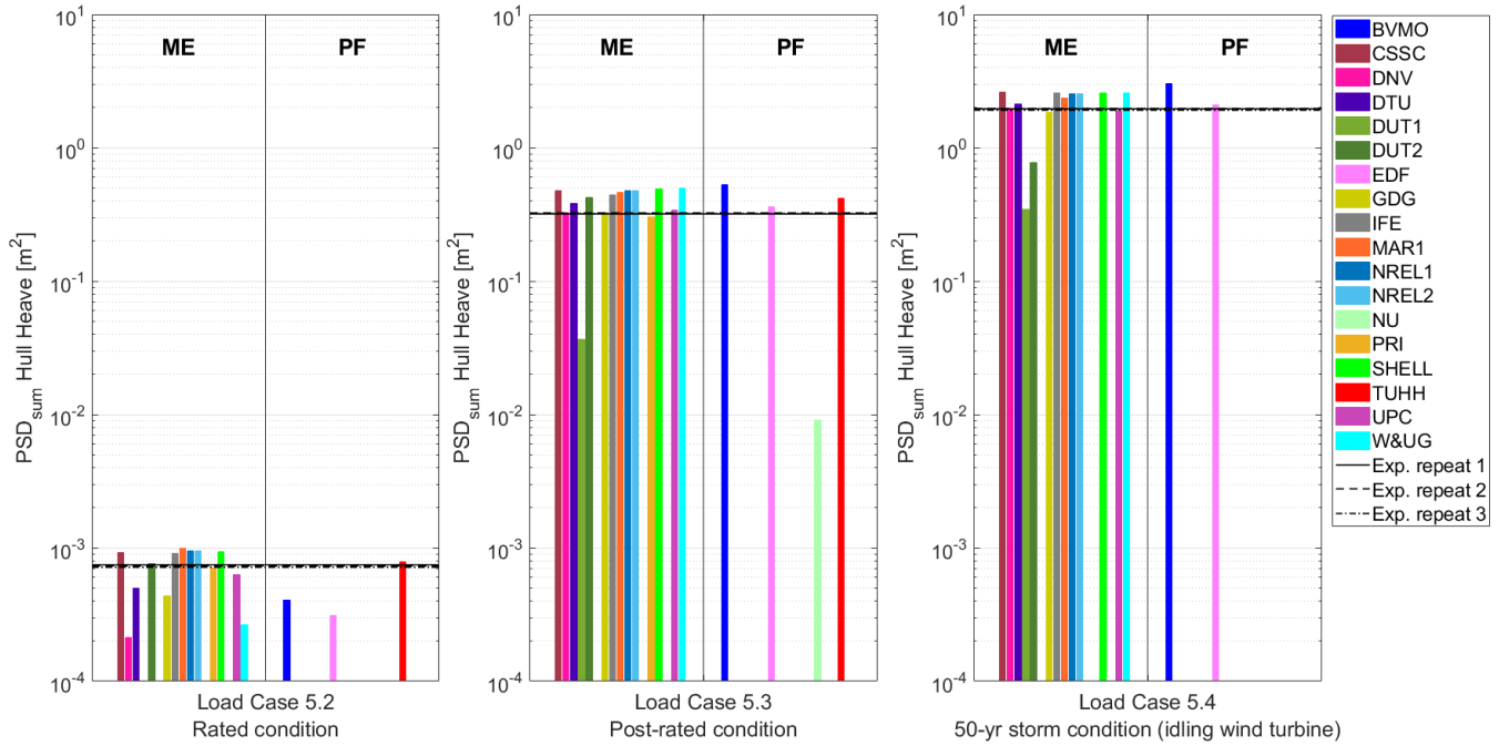
Figure 8: Power spectral density (PSD) sum of the hull heave motion for the combined wind and wave conditions in Load Cases 5.2, 5.3, and 5.4. Outputs sorted out according to the hydrodynamic theory: Morison equation (ME) and potential flow (PF). Vertical axis in logarithmic scale.
