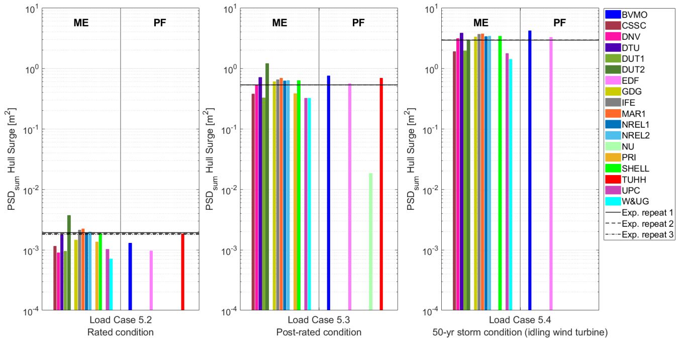
Figure 7: Power spectral density (PSD) sum of the hull surge motion for the combined wind and wave conditions in Load Cases 5.2, 5.3, and 5.4. Outputs sorted out according to the hydrodynamic theory: Morison equation (ME) and potential flow (PF). Vertical axis in logarithmic scale.
