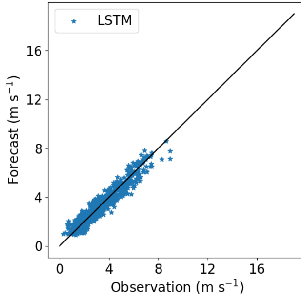
Figure 16. Correlation between forecasted and observed data for the Site 1 with the model trained at Site 3. Height: 100 80 m
