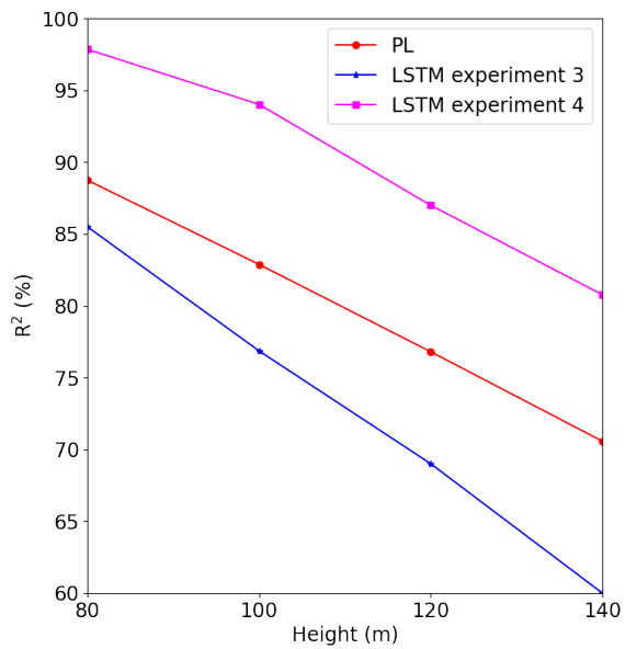
Figure 21. As Fig-15, except Site 3: Comparison for the 60-m wind speed was added to the input dataset PL, Experiment 3 and Experiment 4 estimates
