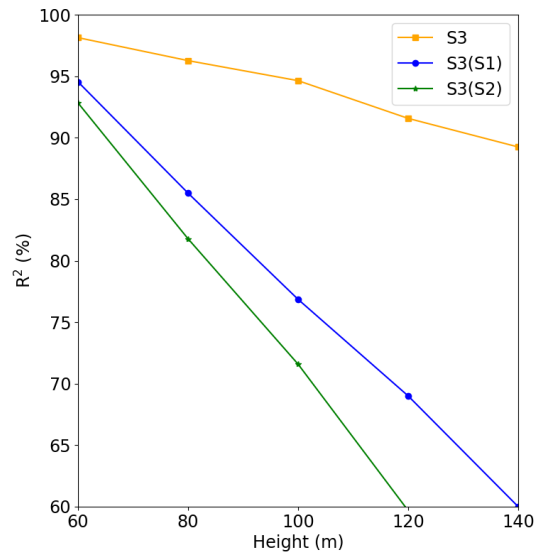
Figure 15. Correlation Comparison between forecasted the Experiment 1 and observed data Experiment 3 , where S3 is the result of the Experiment 1 ; S3(S1) is the forecast for the Site 3 ran with the model of the Site 1; and S3(S2) is the forecast for the Site 3 ran with the model trained at of the Site 3-Height: 80 m]
