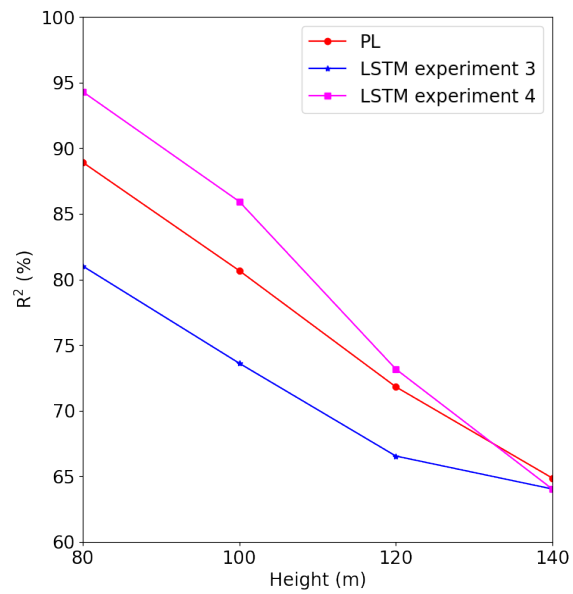
Figure 20. Site 32: Comparison for the PL , Experiment 3 and Experiment 4 estimates
