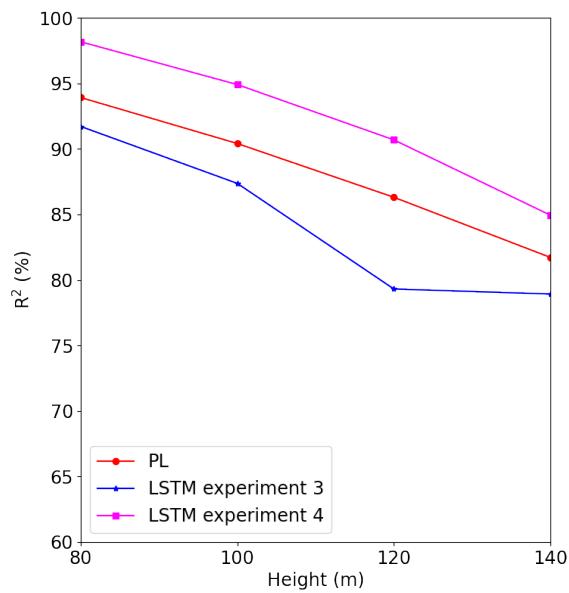
Figure 19. Site 21: Comparison for the PL, Experiment 3 and Experiment 4 estimates
