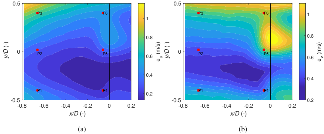
Figure 8. Dual-Doppler reconstruction error for the (a) longitudinal ( e_u ) and (b) lateral ( e_v ) components for the evaluated LES flow field. The markers P1 - P6 indicate regions of interest.
