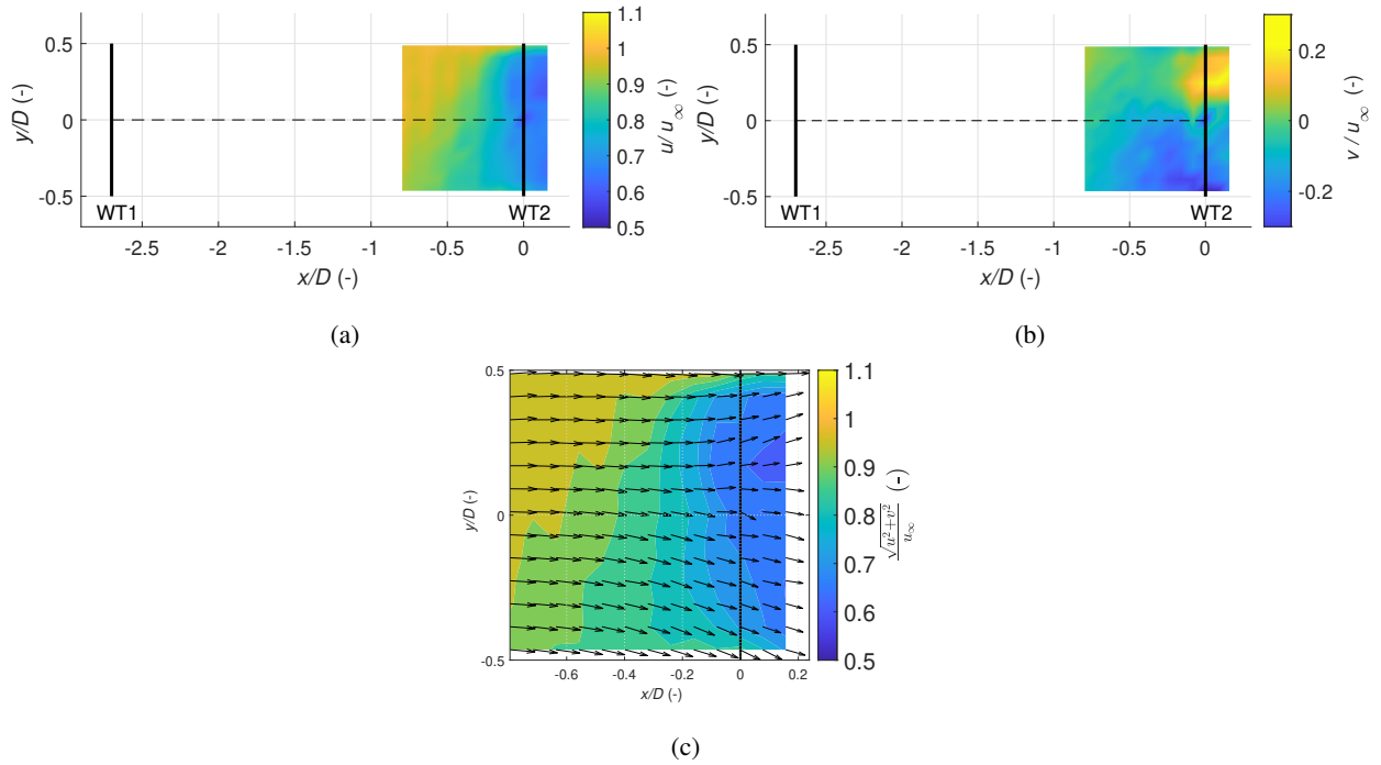
Figure 11. Case 1: Longitudinal (a) and lateral (b) velocities measured while WT1 was not operating and WT2 was operational. In (c), the quiver plot is based on the measured horizontal velocities.
