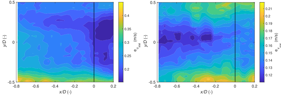
Figure 7. Statistical uncertainty estimated through the margin of error for the (a) u and (b) v components for the evaluated LES flow field.
