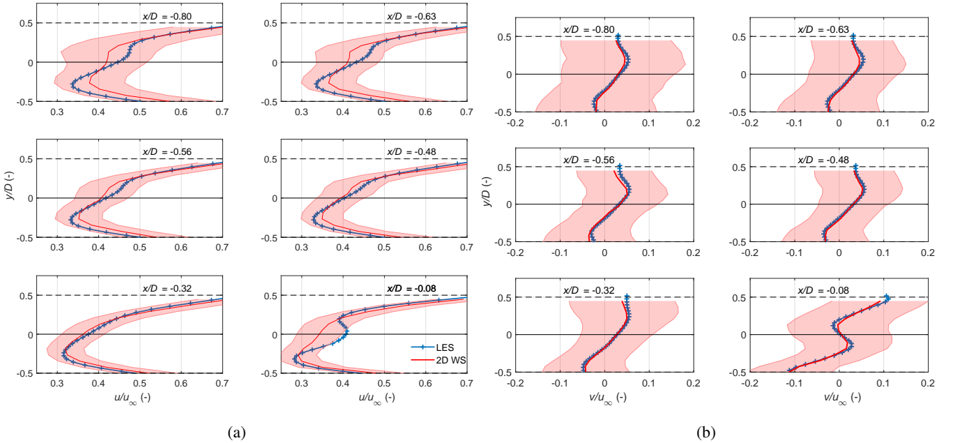
Figure 10. WindScanner estimated velocity profiles (red) of longitudinal (a) and lateral (b) velocities at six upstream cross sections compared against the reference LES (blue). The red shaded area indicate the total combined measurement uncertainty estimated through Eqn. 7 and Eqn. 8 using the local w velocity component.
