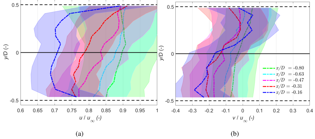
Figure 12. Case 1: Inflow longitudinal (a) and lateral (b) profiles extracted at various positions upstream of WT2. The shaded area represents the total combined measurement uncertainty calculated from the standard uncertainty propagation method ( e_u ) with w = 0.2 m/s, as WT1 was not operational.
