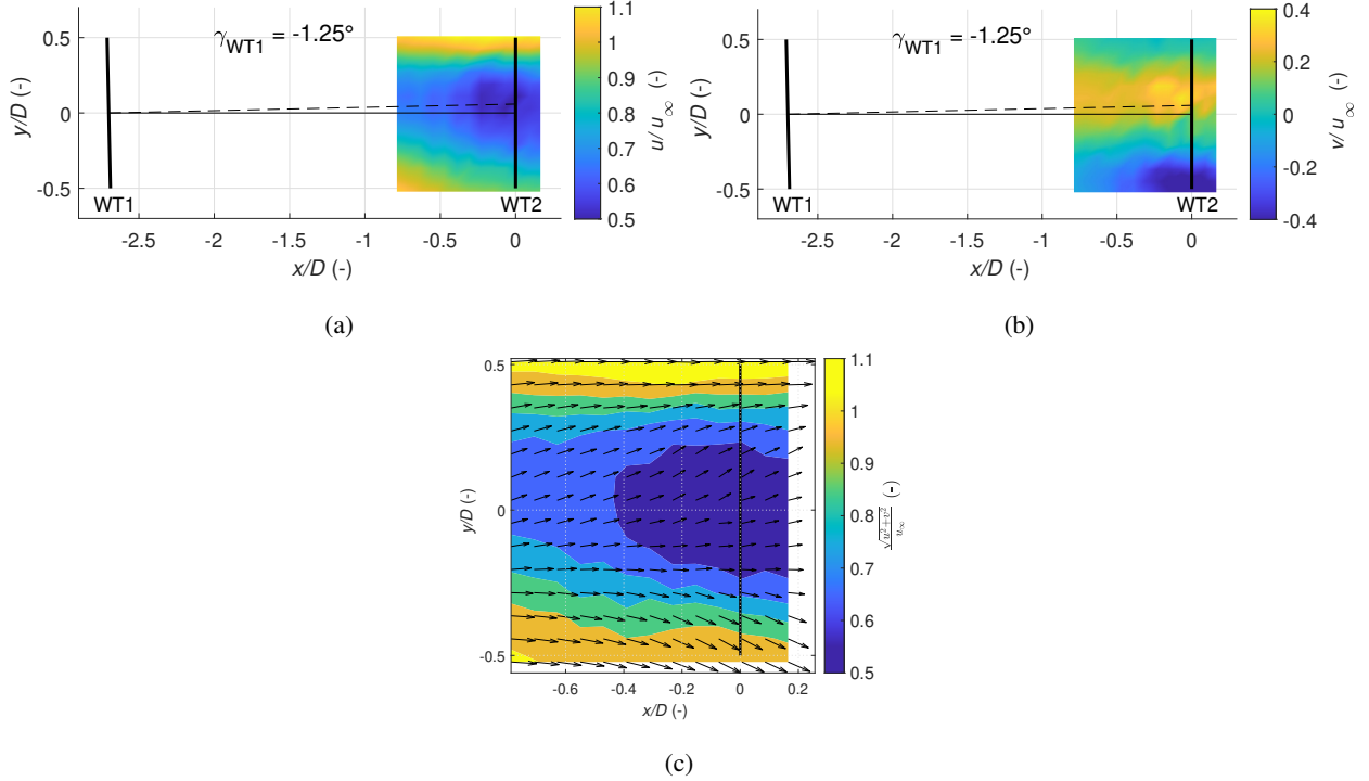
Figure 14. Case 2: Longitudinal (a) and lateral (b) velocities measured for the full wake case. The contour of the magnitude of the horizontal velocity and its vector field is plotted in (c).
