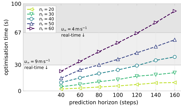
Figure 19. The benchmark for the computational cost of control optimisation shows how the optimisation time scales approximately linearly with the number of steps in the prediction horizon. The computational expense scales quadratically with the wake length, determined by the number of rings n_r in the wake simulation. The horizontal lines provide an indication of the level below which real-time control optimisation is achieved for u_\infty = 4 \text{ m s}^{-1} and u_\infty = 9 \text{ m s}^{-1} with an update every five discrete time steps.
